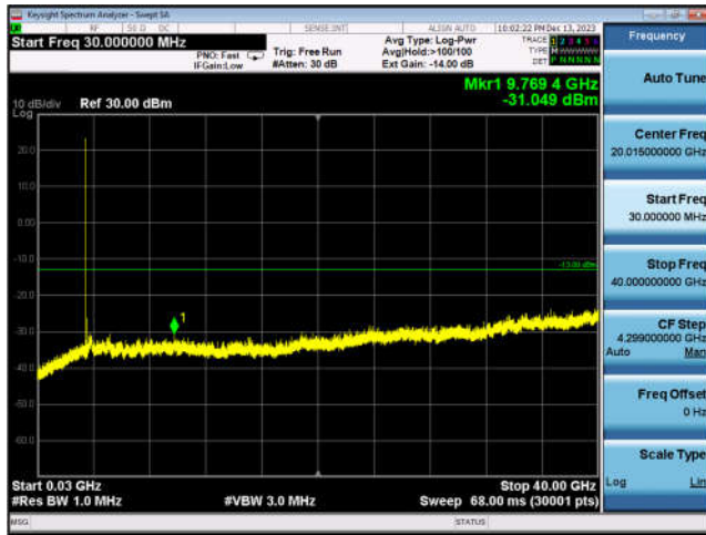
N77_80MHz_DFT-s-OFDM_BPSK_ Edge_1RB_Left_High_CH
