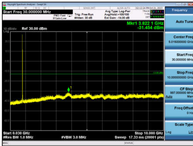
N5_20MHz_DFT-s-OFDM_BPSK_ Edge_1RB_Left_High_CH
