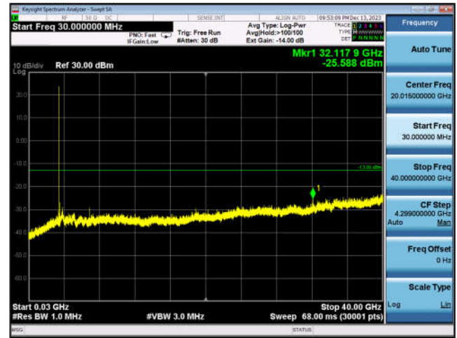
N77_100MHz_DFT-s-OFDM_BPSK_ Edge_1RB_Left_Mid_CH
