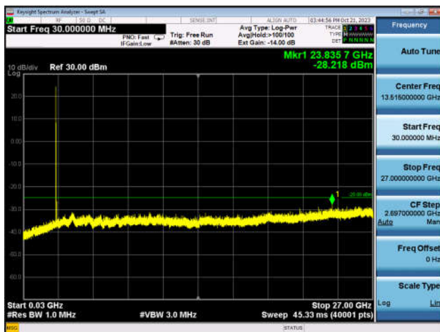
N41_100MHz_DFT-s-OFDM_BPSK_ Edge_1RB_Left_Mid_CH
