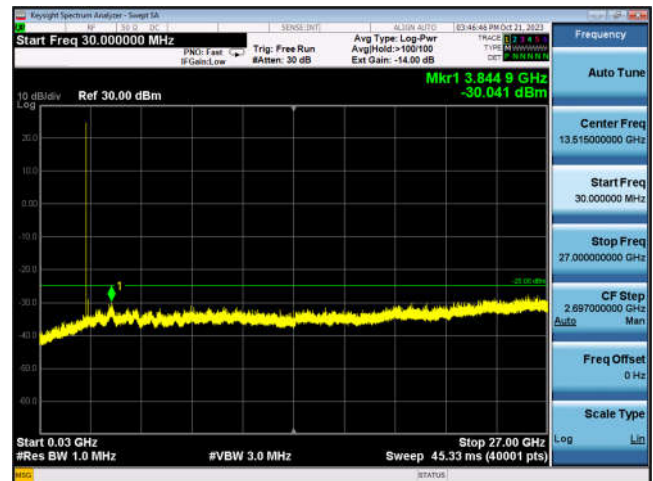
N41_100MHz_DFT-s-OFDM_BPSK_ Edge_1RB_Left_High_CH
