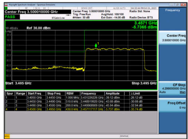
N78_40MHz_DFT-s-OFDM_PI/2-BPSK_Edge_ Outer_Full_High_CH
