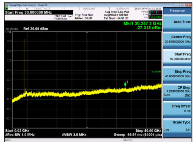
N78_80MHz_DFT-s-OFDM_BPSK_ Edge_1RB_Left_Mid_CH
