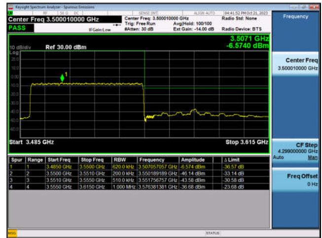
N78_80MHz_DFT-s-OFDM_PI/2-BPSK_Edge_ Outer_Full_Low_CH
