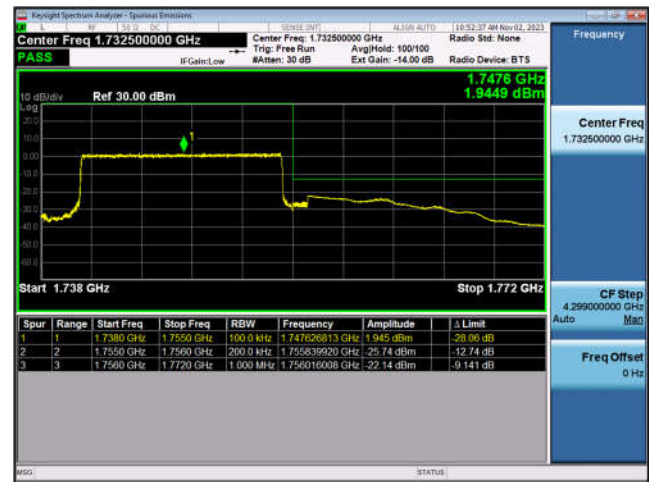
LTE Band 4-20MHz-QPSK-LCH-100RB#0
