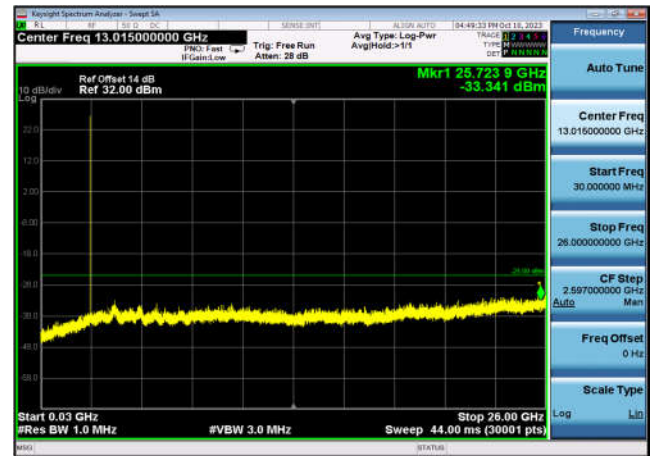
FDD07_HighRange_10MHz_30MHz~26GHz
