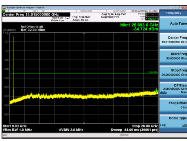
FDD17_MidRange_10MHz_30MHz~26GHz
