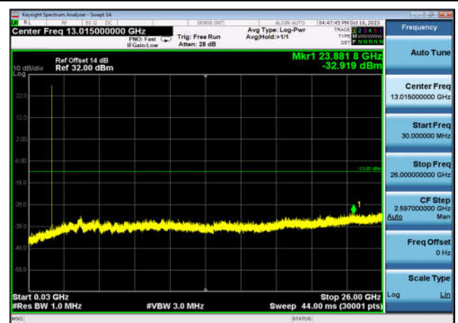
FDD04_HighRange_10MHz_30MHz~26GHz
