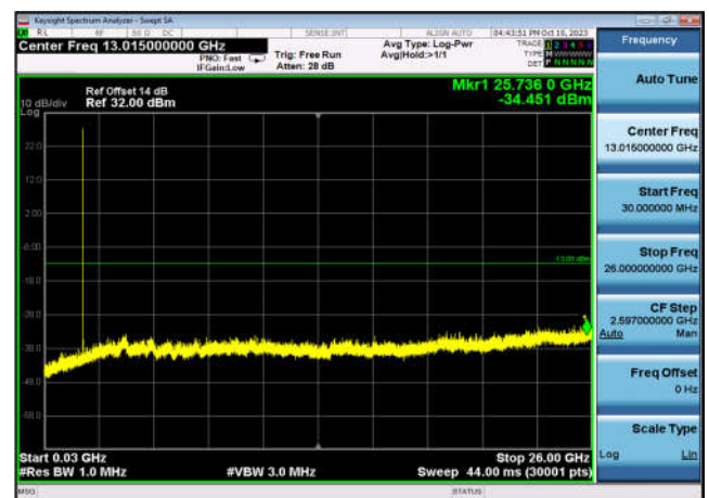
FDD04_LowRange_10MHz_30MHz~26GHz
