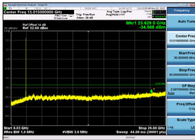
TDD41_HighRange_20MHz_30MHz~26GHz
