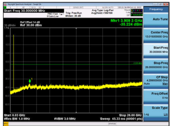
FDD17_LowRange_10MHz_30MHz~26GHz
