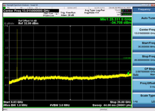
FDD04_MidRange_10MHz_30MHz~26GHz
