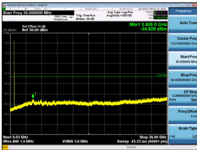
FDD12_HighRange_10MHz_30MHz~26GHz
