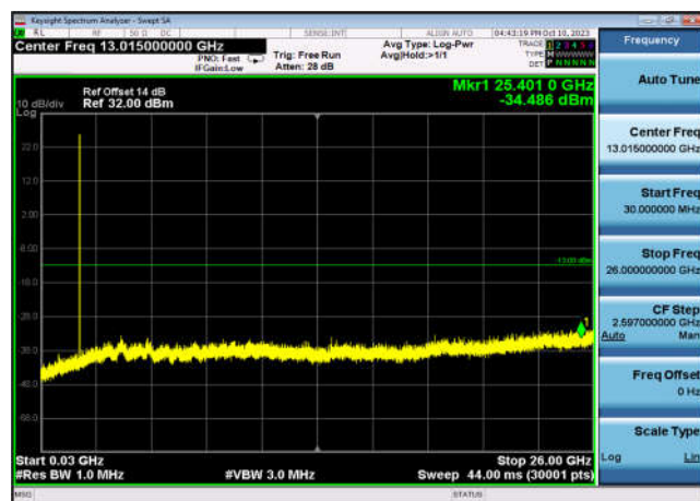
FDD02_HighRange_10MHz_30MHz~26GHz
