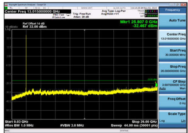
TDD41_MidRange_20MHz_30MHz~26GHz
