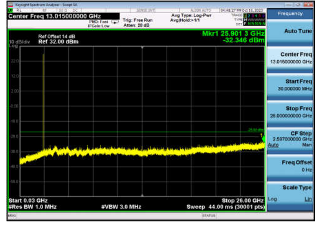
FDD07_HighRange_10MHz_30MHz~26GHz
