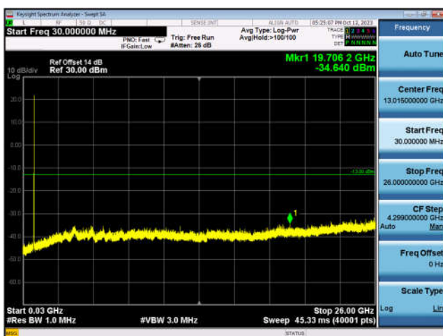
FDD07_MidRange_10MHz_30MHz~26GHz
