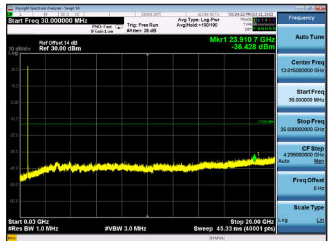
FDD07_LowRange_10MHz_30MHz~26GHz
