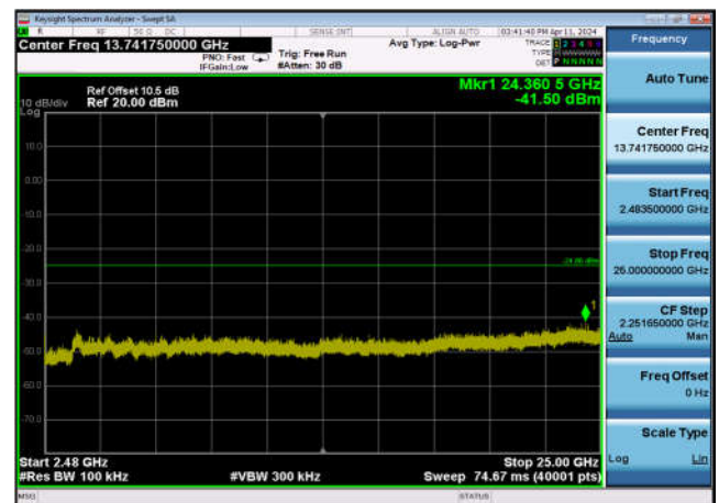
,Plot 4,2483.5MHz~25000MHz-802.11n(20 MHz),2437MHz,Ant12
