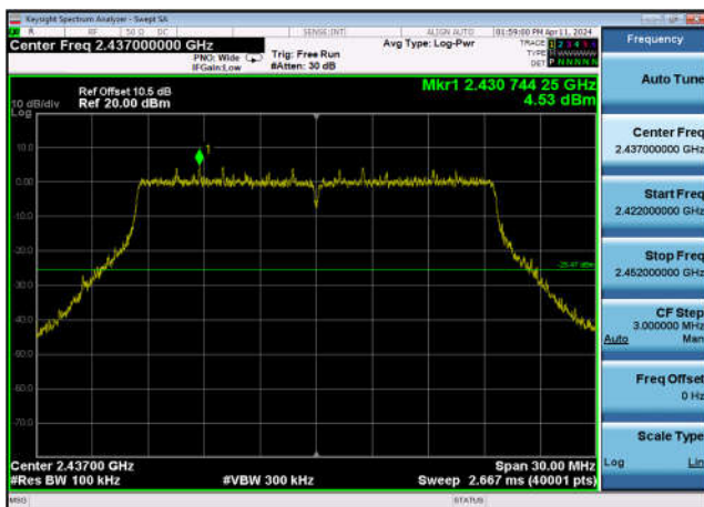
,Plot 1,Reference Level-802.11ax(20MHz z),2437MHz,Ant13
