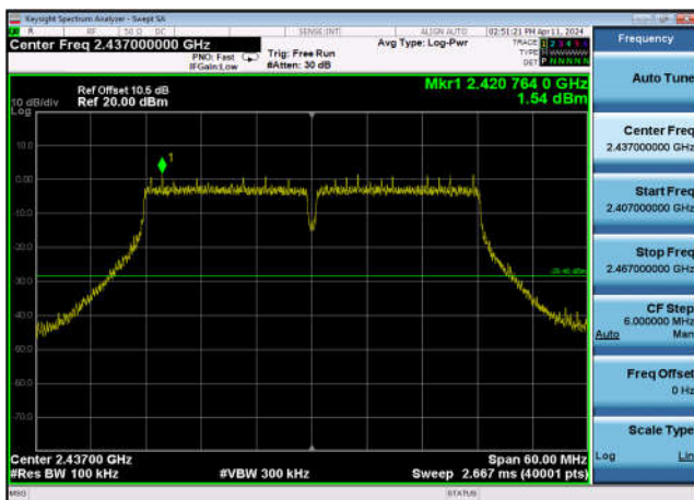
,Plot 1,Reference Level-802.11n(40MHz ),2437MHz,Ant13
