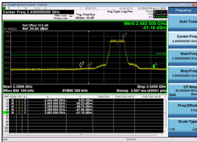
,Plot 2,Band Edge-802.11ax(20MHz) ,2437MHz,Ant13
