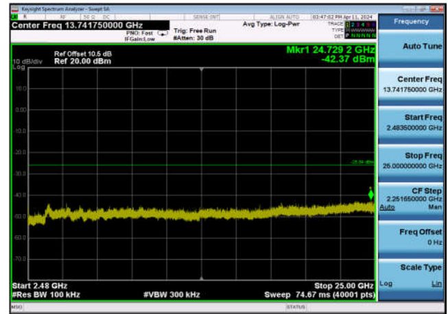
,Plot 1,Reference Level-802.11n(40MHz ),2422MHz,Ant12
