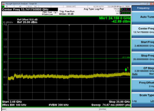
,Plot 4,2483.5MHz~25000MHz-802.11n(20 MHz),2437MHz,Ant13
