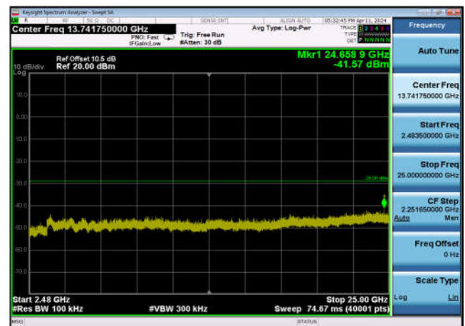
,Plot 4,2483.5MHz~25000MHz-802.11n(40 MHz),2437MHz,Ant12
