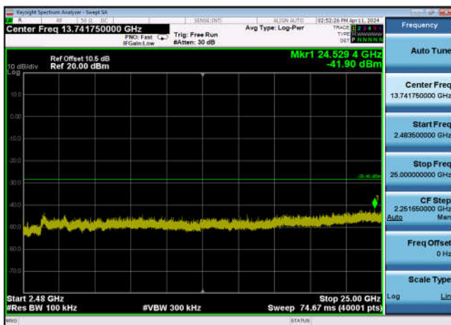
,Plot 4,2483.5MHz~25000MHz-802.11n(40 MHz),2437MHz,Ant13
