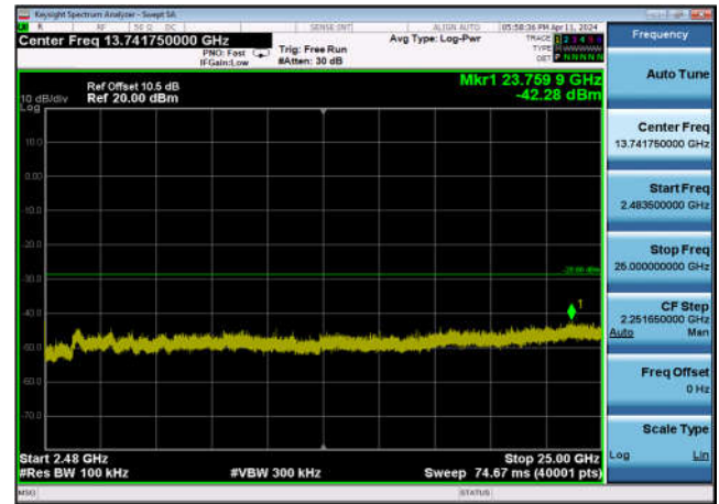
,Plot 1,Reference Level-802.11ax(20MHz z),2412MHz,Ant12
