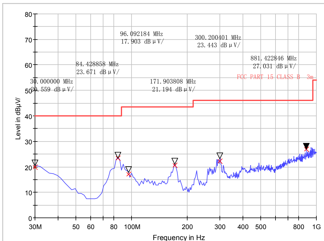
EMI Sweep-3M(30-1G)
