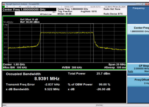
FDD02_MidRange_15_1880_QPSK
