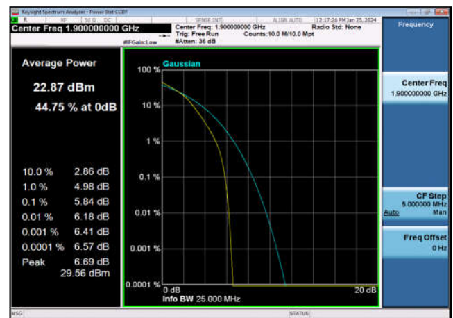
FDD02_HighRange_20MHz_1900_fullIRB _Q16
