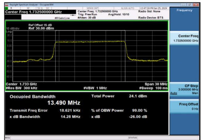
FDD04_MidRange_20_1732.5_Q16
