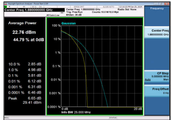
FDD02_HighRange_20MHz_1900_fullIRB _Q16
