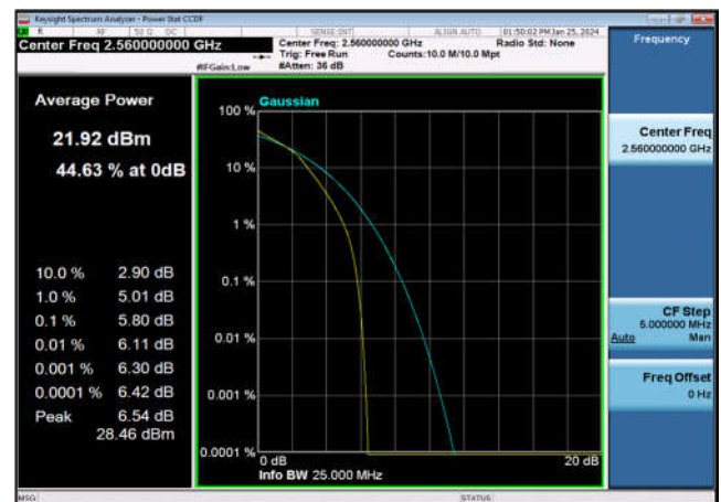
FDD07_HighRange_20MHz_2560_fullIRB _Q16
