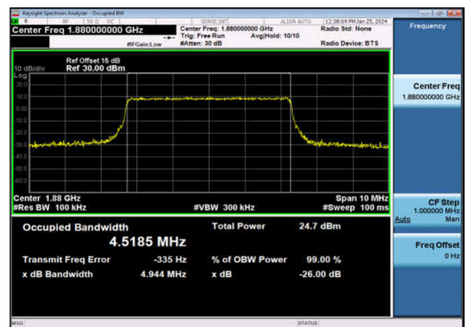
FDD02_MidRange_5_1880_Q16
