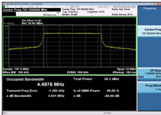
FDD12_MidRange_10_707.5_QPSK
