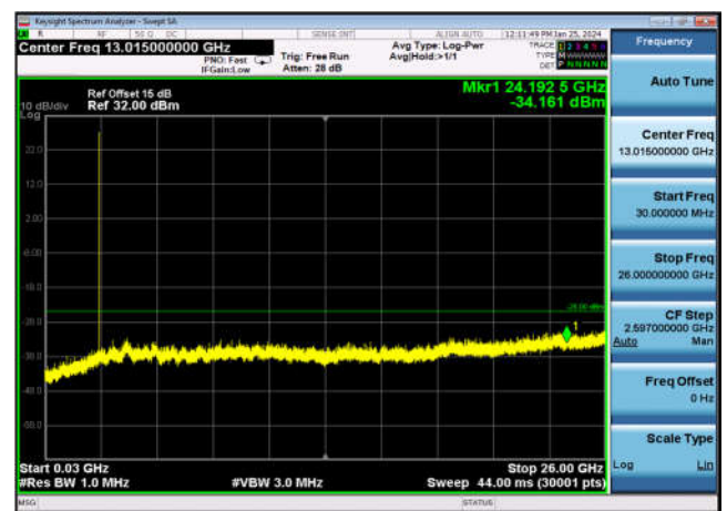
TDD41_LowRange_20MHz_30MHz~26GHz
