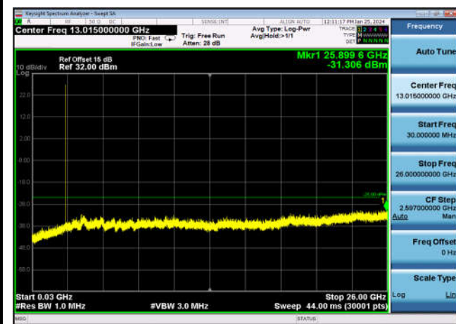
FDD07_HighRange_20MHz_30MHz~26GHz
