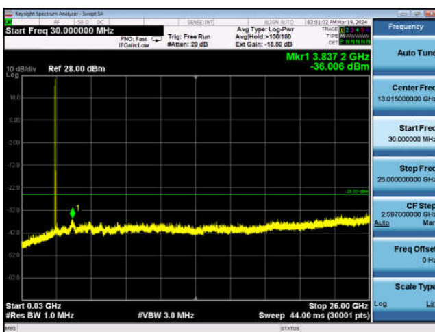
LTE Band 7C_MidRange -20MHz+20MHz_30MHz~26GHz
