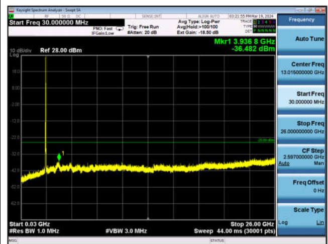
LTE Band 7C_HighRange -20MHz+20MHz_30MHz~26GHz
