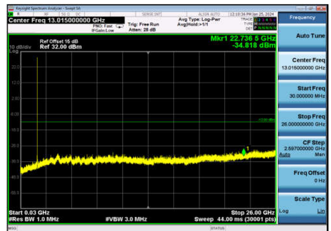
FDD04_HighRange_20MHz_30MHz~26GHz
