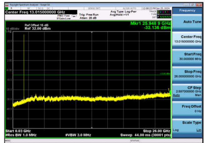
FDD04_LowRange_20MHz_30MHz~26GHz
