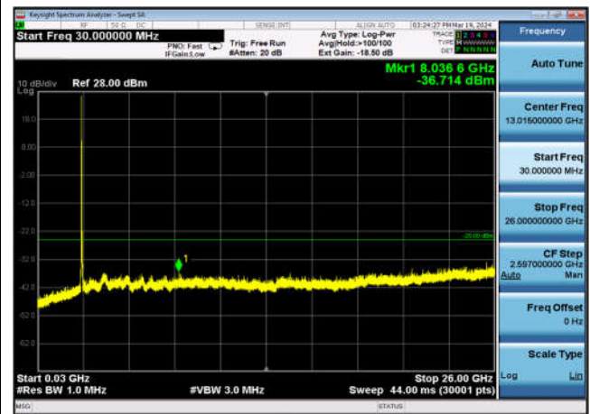
LTE Band 7C_HighRange -20MHz+20MHz_30MHz~26GHz
