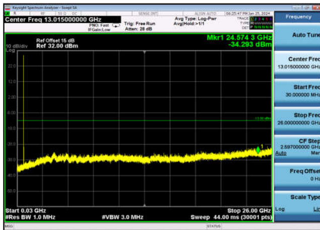
FDD17_LowRange_10MHz_30MHz~26GHz
