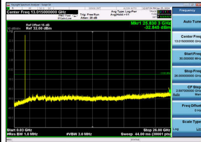
FDD02_HighRange_20MHz_30MHz~26GHz
