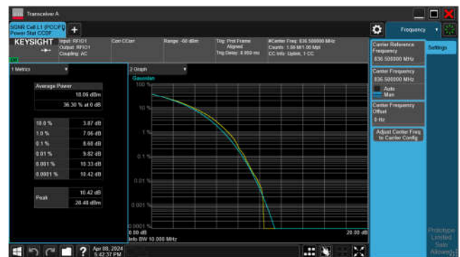
Band n5_20MHz_CP-OFDM_256QAM_ Outer_Full_Mid_CH
