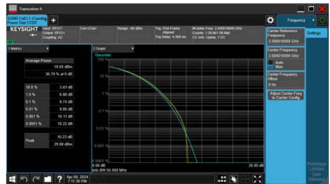
Band n77_60MHz_CP-OFDM_256QAM_ Outer_Full_Mid_CH
