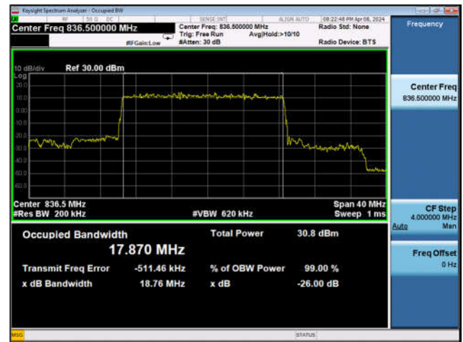
Band n5_20MHz_DFT-s-OFDM_QPSK_ Outer_Full_Mid_CH
