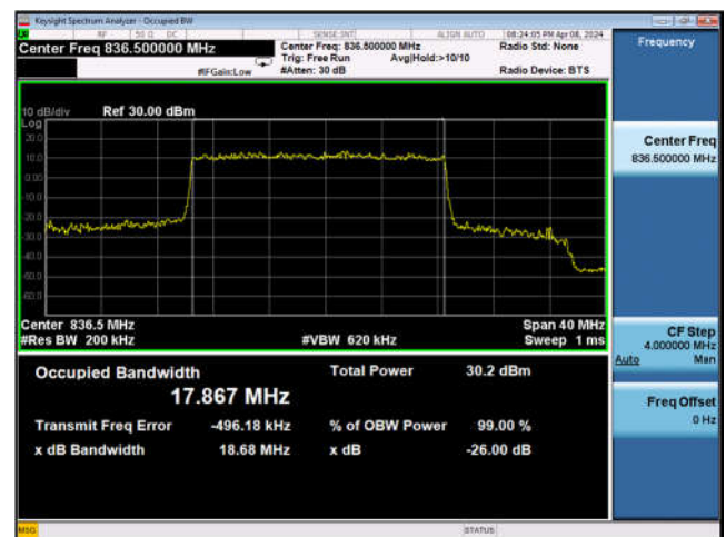
Band n5_20MHz_DFT-s-OFDM_16QAM_ Outer_Full_Mid_CH
