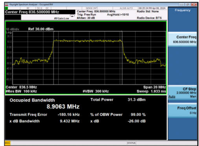
Band n5_10MHz_DFT-s-OFDM_QPSK_ Outer_Full_Mid_CH
