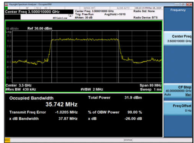
Band n77_40MHz_DFT-s-OFDM_QPSK_ Outer_Full_Mid_CH
