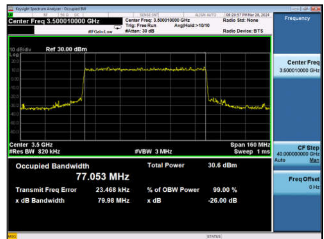
Band n77_80MHz_DFT-s-OFDM_16QAM_ Outer_Full_Mid_CH
