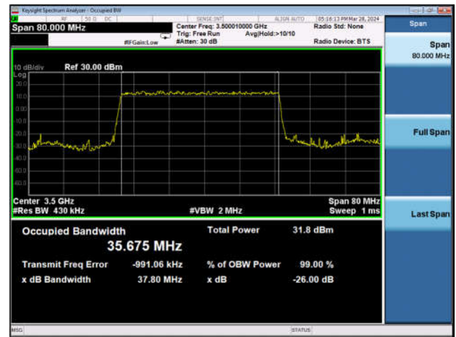
Band n78_40MHz_DFT-s-OFDM_QPSK_ Outer_Full_Mid_CH
