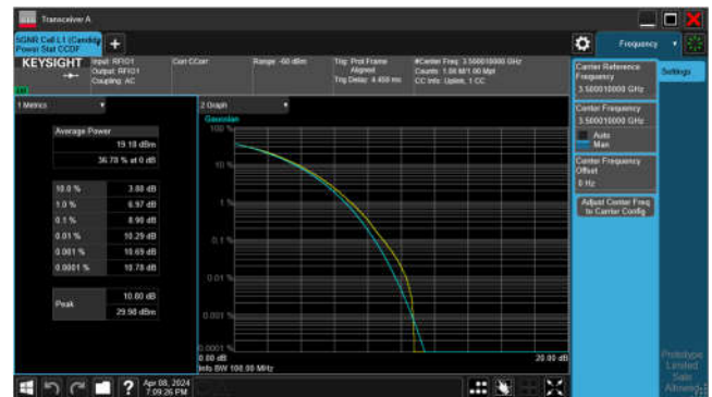
Band n77_100MHz_CP-OFDM_256QAM_ Outer_Full_Mid_CH
