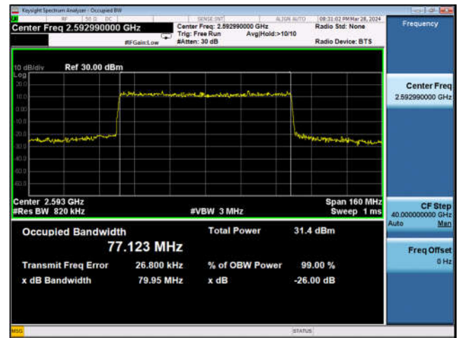
Band n41_80MHz_DFT-s-OFDM_QPSK_ Outer_Full_Mid_CH
