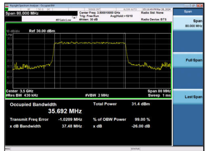
Band n78_40MHz_DFT-s-OFDM_16QAM_ Outer_Full_Mid_CH
