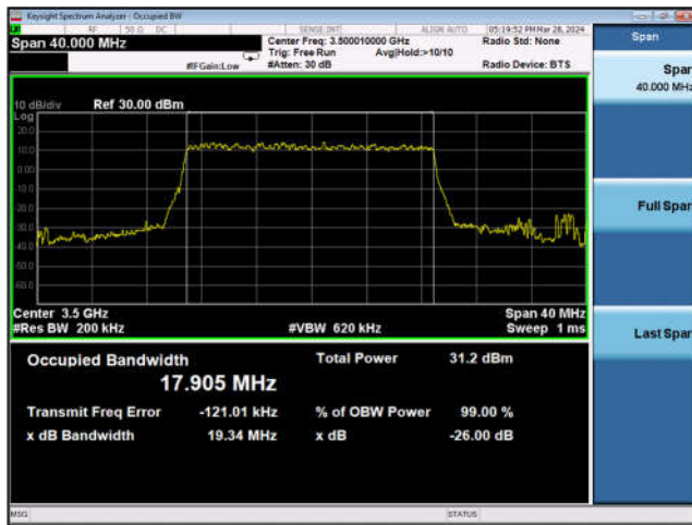
Band n78_20MHz_DFT-s-OFDM_QPSK_ Outer_Full_Mid_CH
