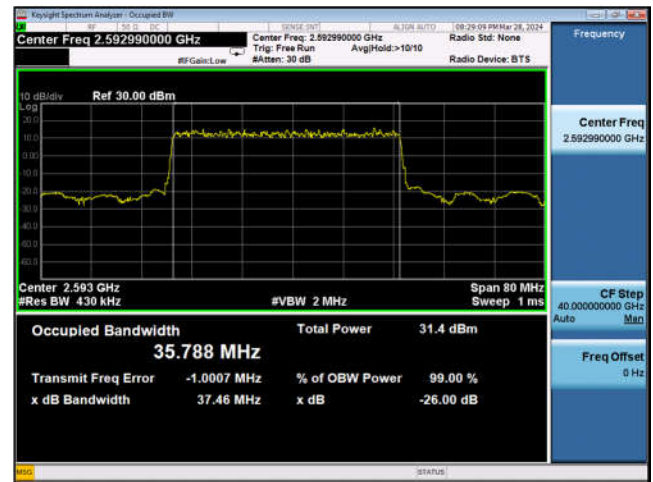
Band n41_40MHz_DFT-s-OFDM_QPSK_ Outer_Full_Mid_CH
