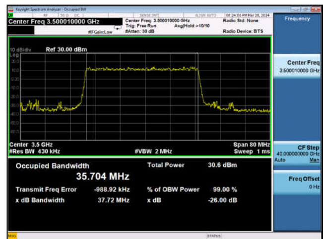
Band n77_40MHz_DFT-s-OFDM_16QAM_ Outer_Full_Mid_CH
