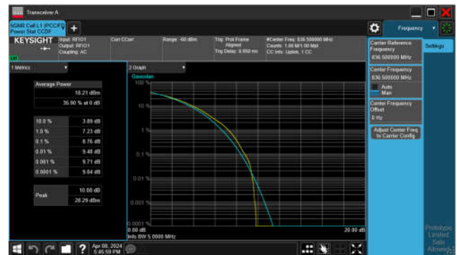
Band n5_10MHz_CP-OFDM_256QAM_ Outer_Full_Mid_CH
