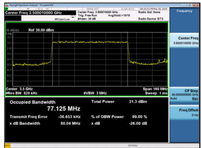
Band n77_80MHz_DFT-s-OFDM_QPSK_ Outer_Full_Mid_CH
