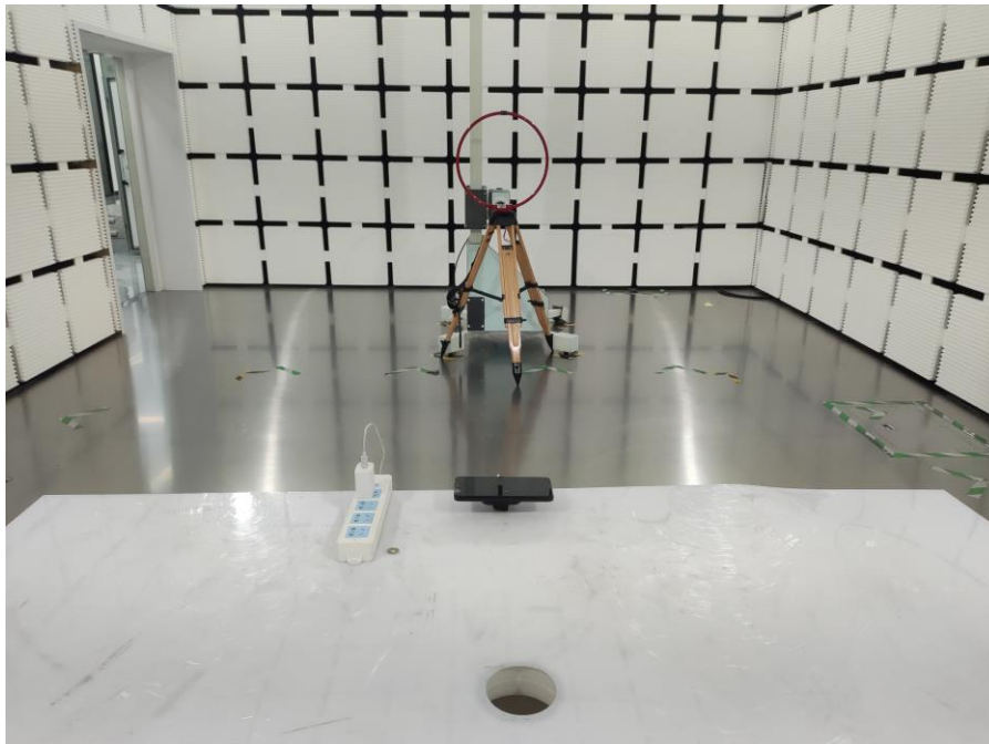
Radiation (9KHz-30MHz)
