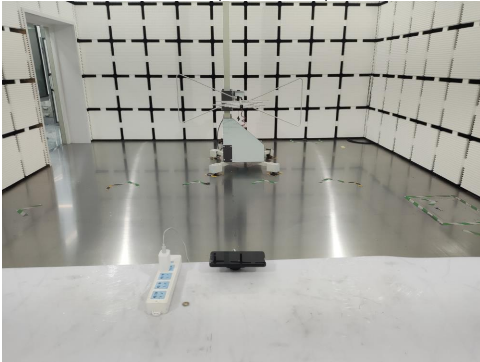
Radiation (30MHz-1000MHz)
