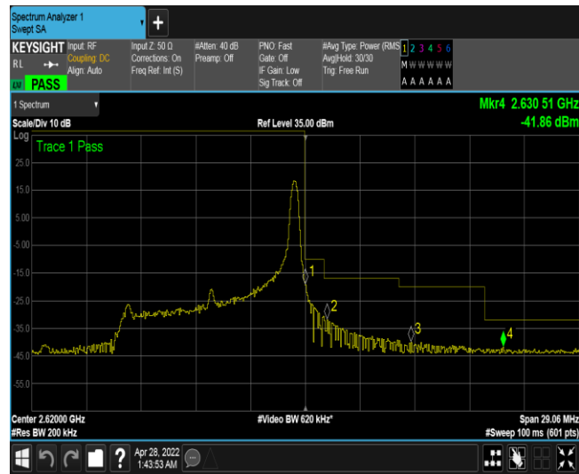
Band38-10MHz-QPSK-38200-50RB#0
