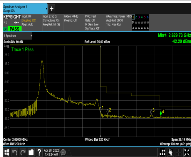
Band38-10MHz-16QAM-38200-1RB#49
