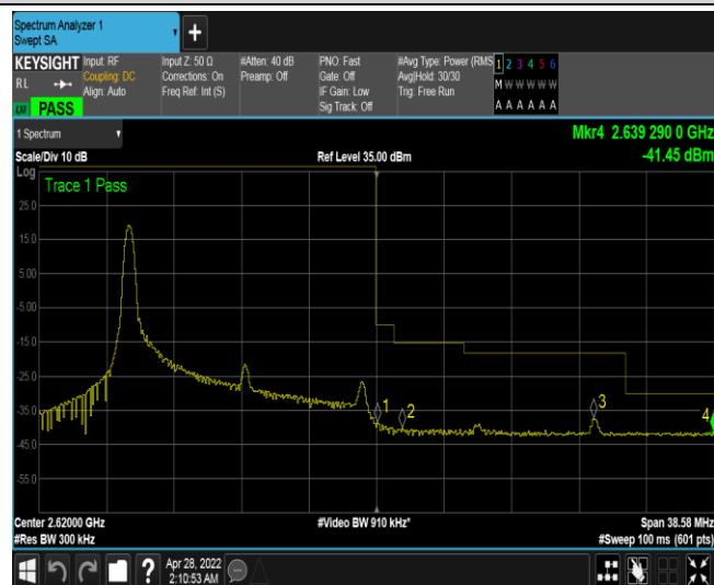
Band38-15MHz-16QAM-38175-1RB#0
