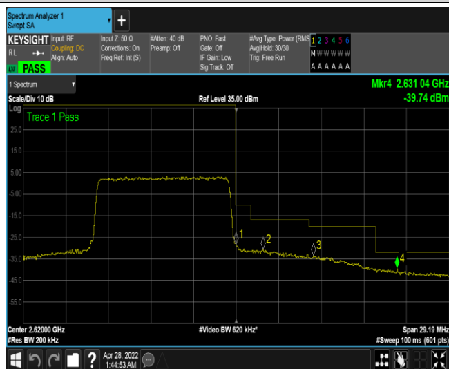
Band38-10MHz-16QAM-38200-50RB#0
