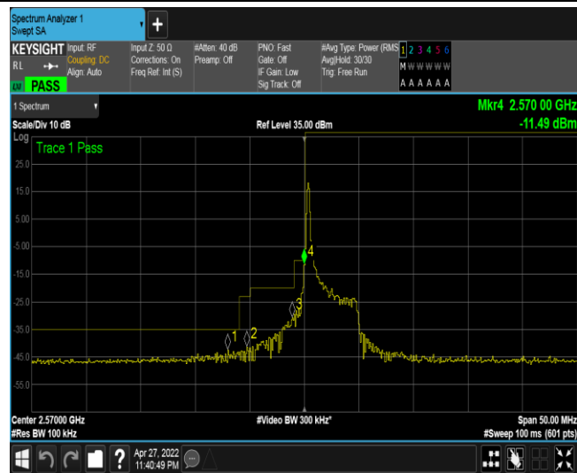
Band38-5MHz-16QAM-37775-1RB#24
