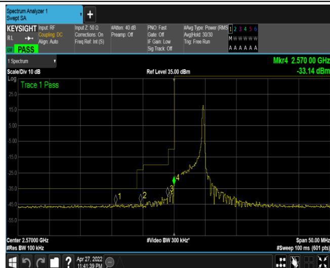
Band38-5MHz-16QAM-37775-25RB#0
