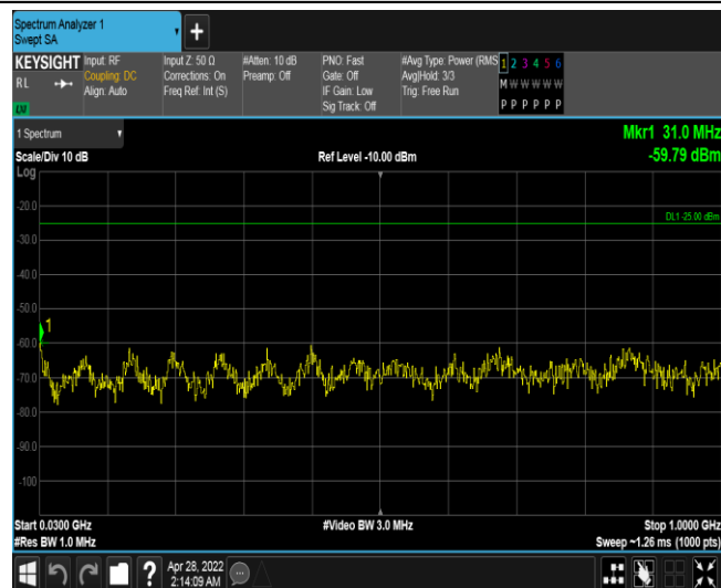
Band38-15MHz-QPSK-38000-1RB#0-Range1:30~1000MHz
