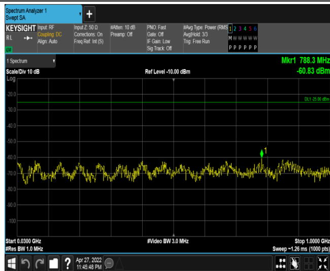
Band38-5MHz-16QAM-37775-1RB#0-Range1:30~1000MHz
