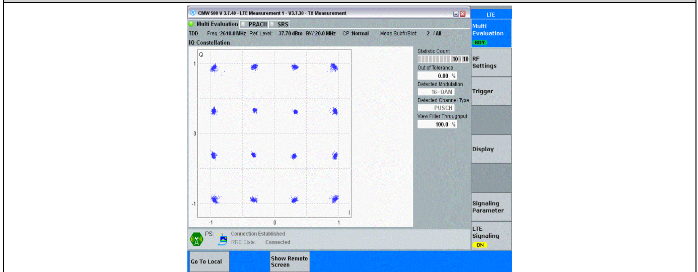
Band38-20MHz-16QAM-38150-100RB#0
