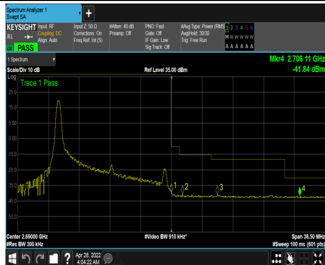
Band41-15MHz-QPSK-41515-1RB#74
