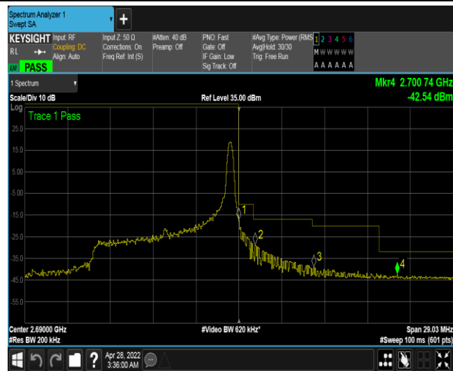
Band41-10MHz-QPSK-41540-50RB#0
