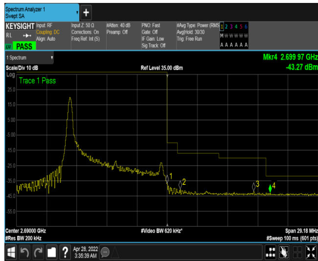
Band41-10MHz-16QAM-41540-1RB#49
