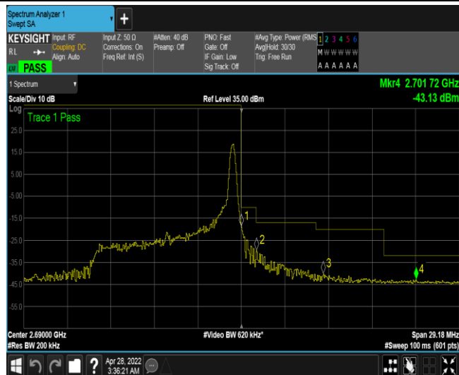
Band41-10MHz-16QAM-41540-50RB#0
