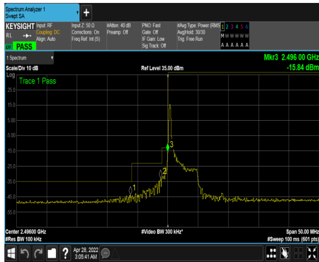
Band41-5MHz-16QAM-39675-1RB#24
