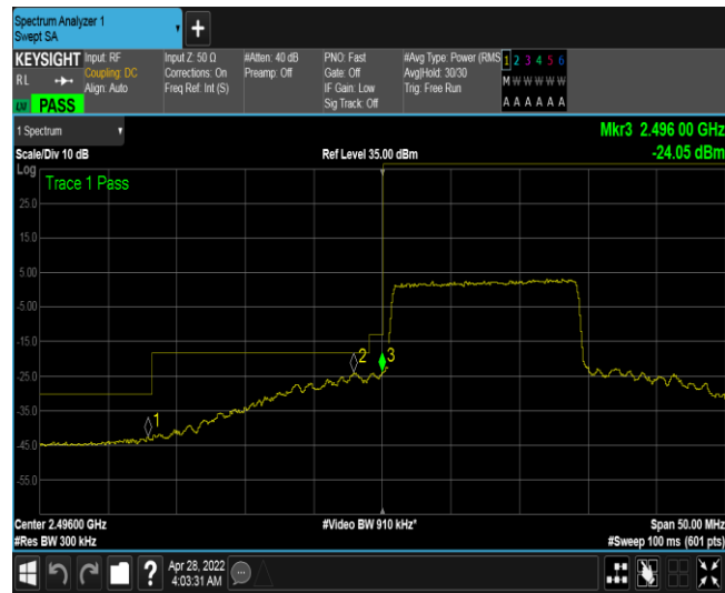
Band41-15MHz-QPSK-41515-1RB#0
