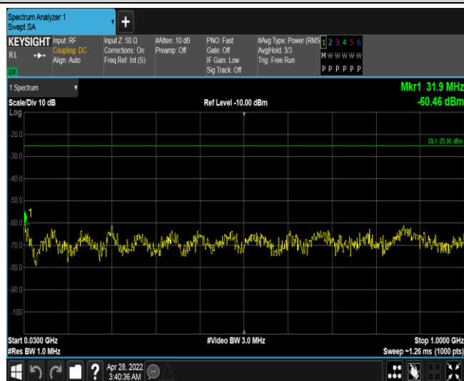
Band41-10MHz-QPSK-41540-1RB#0-Range1:30~1000MHz
