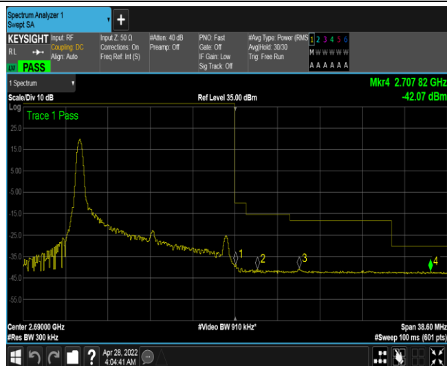
Band41-15MHz-16QAM-41515-1RB#0
