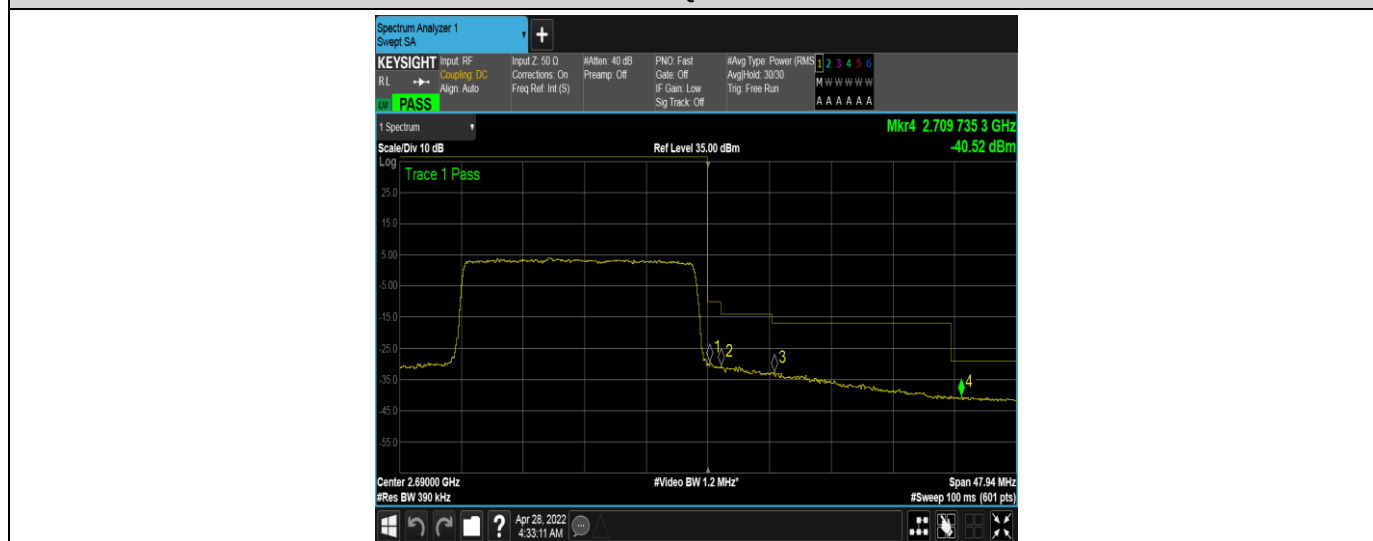
Band41-20MHz-16QAM-41490-100RB#0
