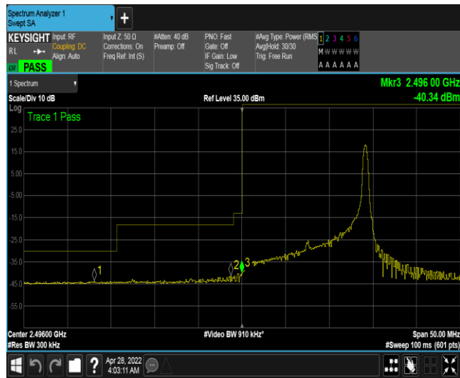
Band41-15MHz-16QAM-39725-75RB#0
