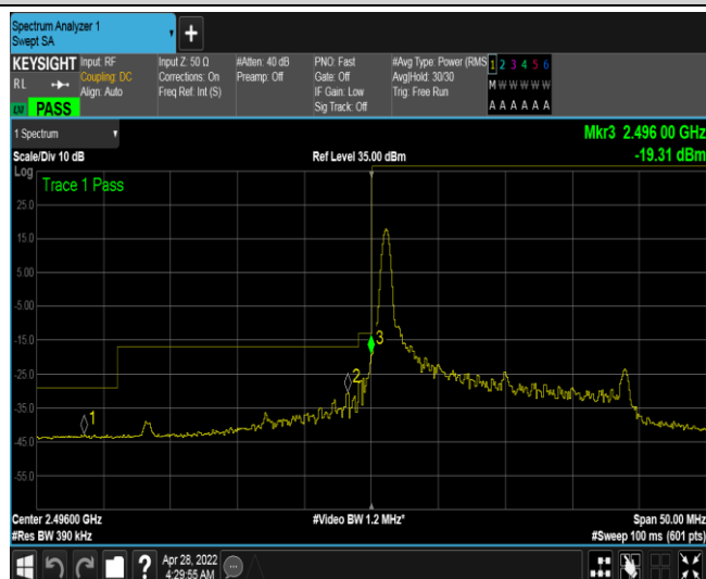
Band41-20MHz-16QAM-39750-1RB#99
