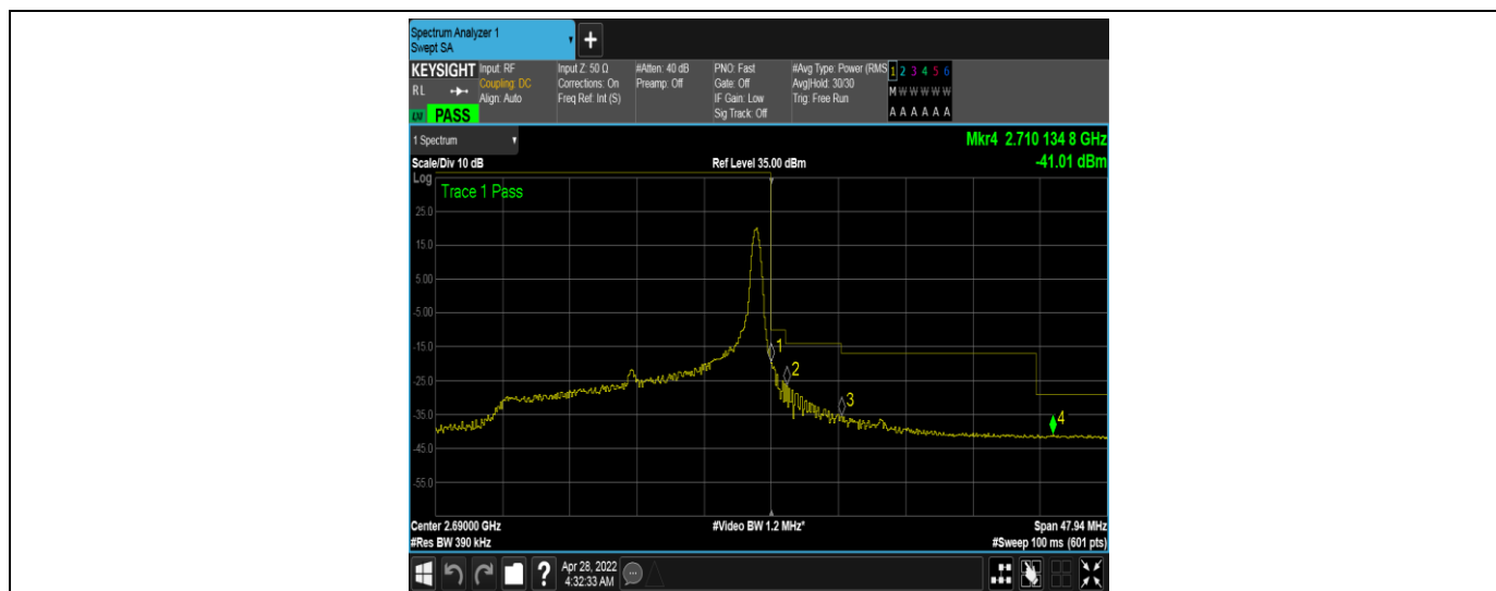
Band41-20MHz-16QAM-41490-100RB#0
