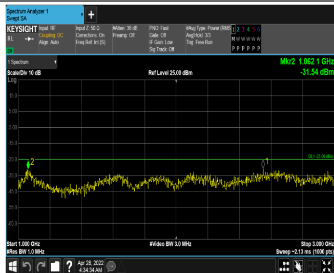
Band41-20MHz-16QAM-39750-1RB#0-Range2:1000~3000MHz
