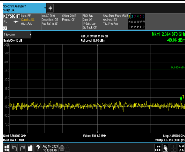
Band40-5MHz-16QAM-38750-1RB#0-Range12:2360~2365MHz
