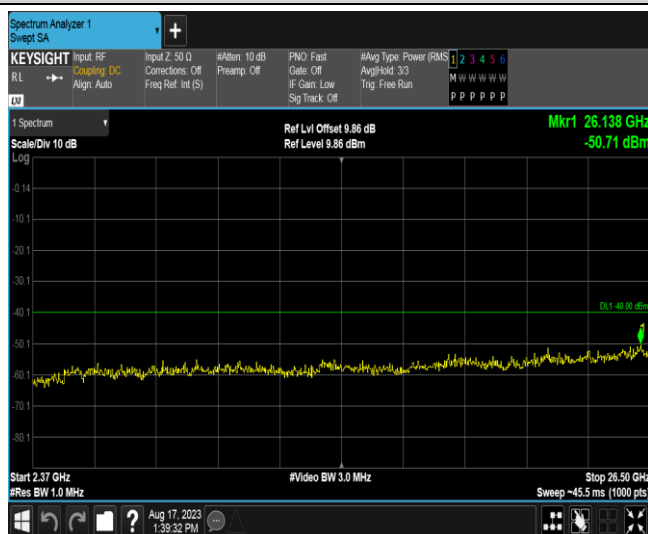
Band40-5MHz-16QAM-39225-1RB#0-Range13:2365~26500MHz
