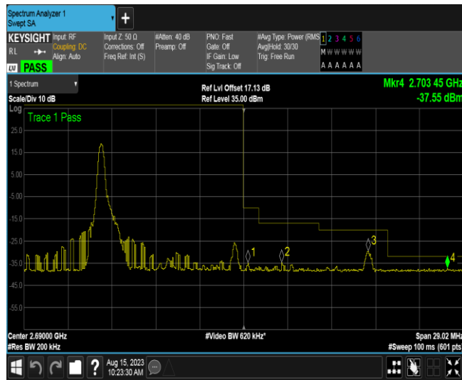
Band41-10MHz-16QAM-41540-1RB#49
