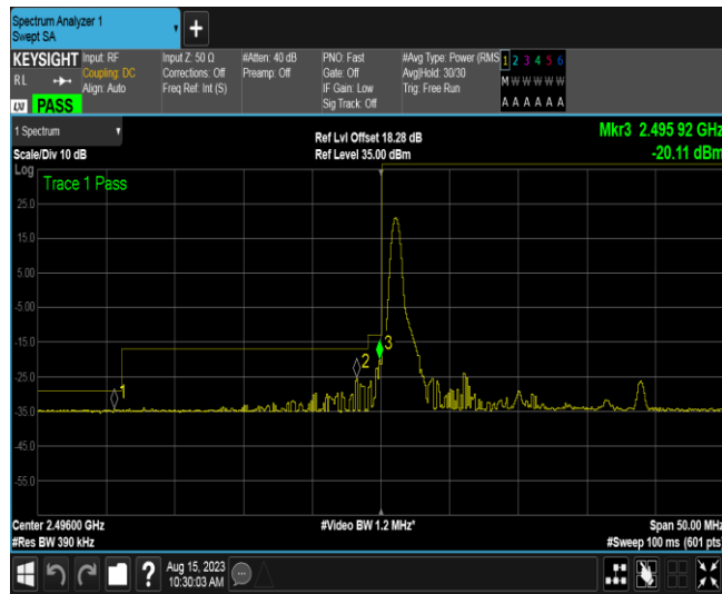
Band41-20MHz-QPSK-39750-1RB#99
