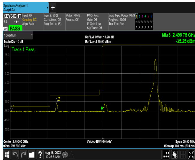
Band41-15MHz-16QAM-39725-75RB#0
