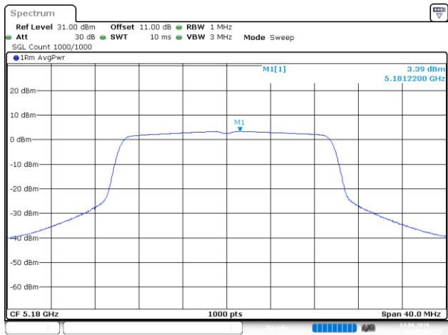
802.11ax20_5180MHz_RU_Full
