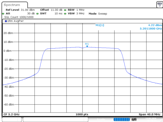
802.11ax20_5200MHz_RU_Full
