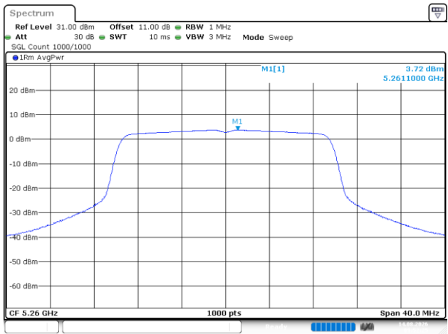
802.11ax20_5260MHz_RU_Full
