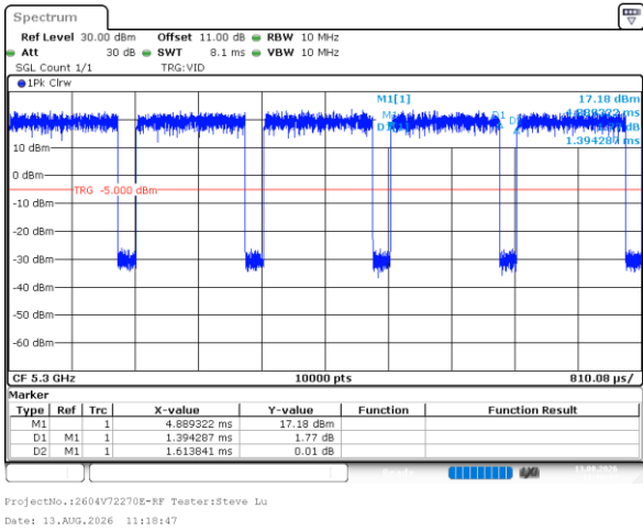
802.11a_5300MHz
