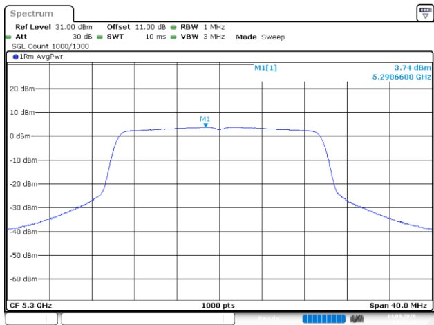
802.11ax20_5300MHz_RU_Full
