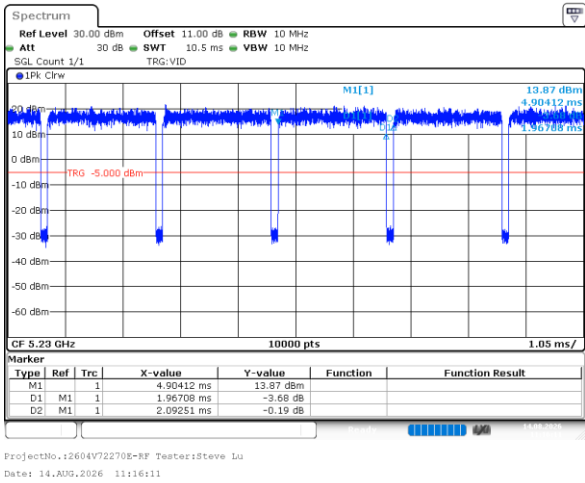
802.11ax40_5230MHz_RU_Full
