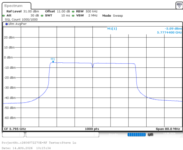
802.11ax40_5795MHz_RU_Full
