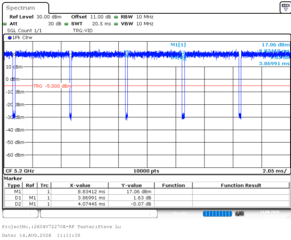
802.11ax20_5200MHz_RU_Full
