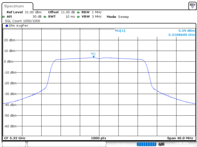
802.11ax20_5320MHz_RU_Full
