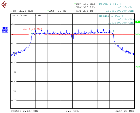
TX 11g channel 6
