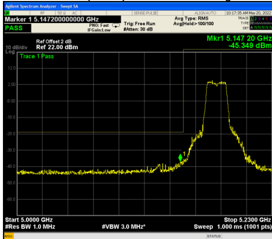
802.11n(HT40) U-NII-1 Band edge-left side
