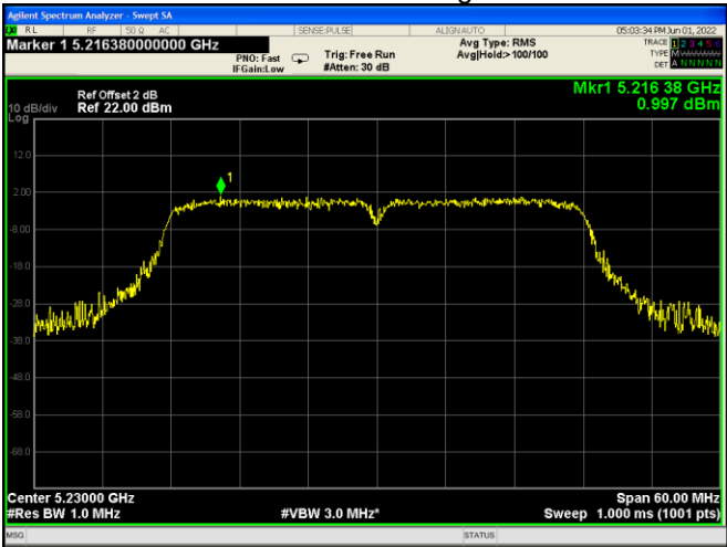
802.11n HT40 U-NII-1 High channel
