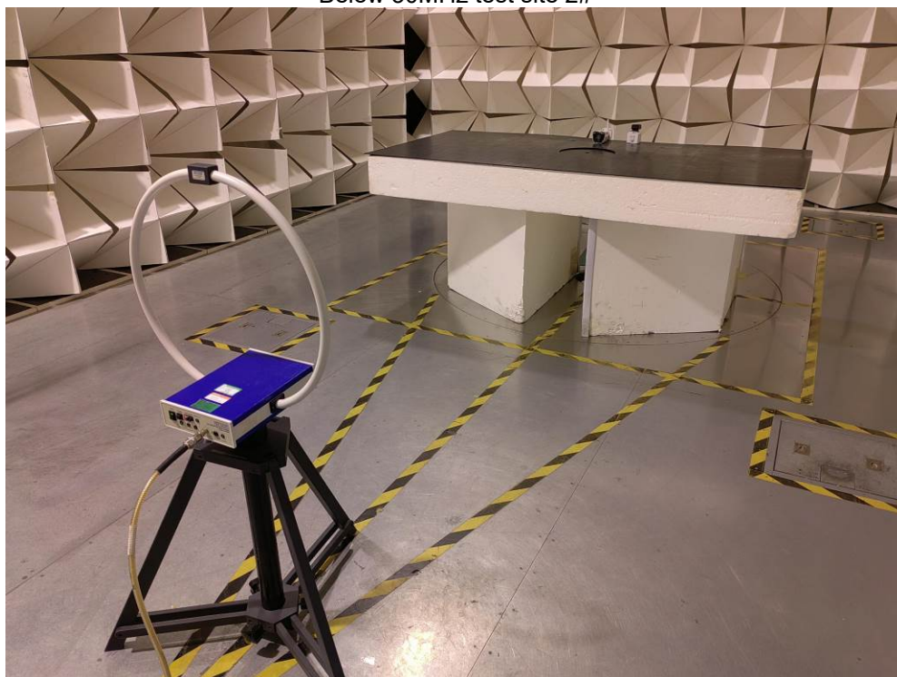
Below 30MHz test site 2#
