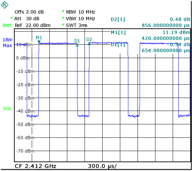
Wi-Fi 802.11n-HT20
