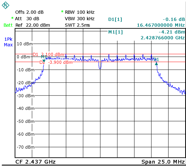
TX 11g channel 6
