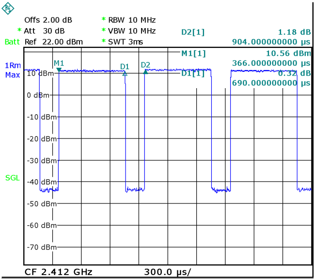
Wi-Fi 802.11g
