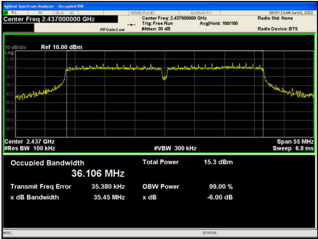
TX 11n HT40 channel 6
