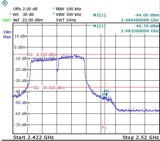
TX 11n HT40: Band edge-right side
