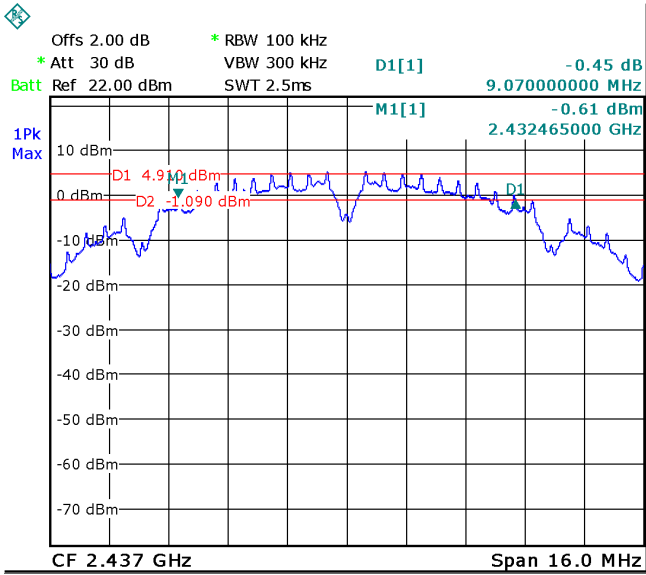
TX 11b channel 6
