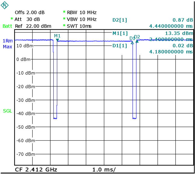
Wi-Fi 802.11b
