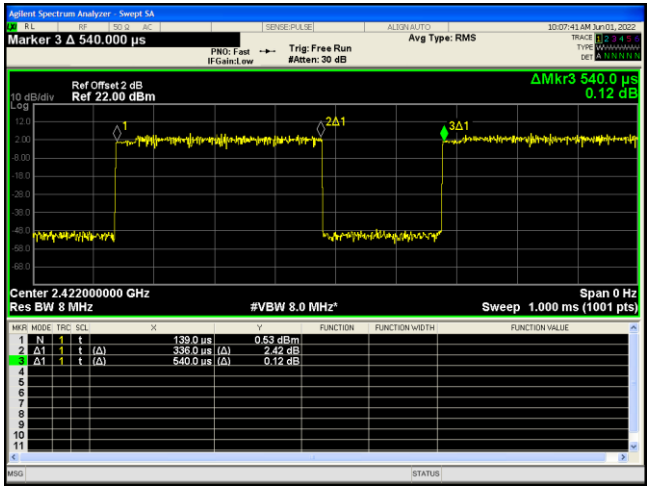
Wi-Fi 802.11n-HT40
