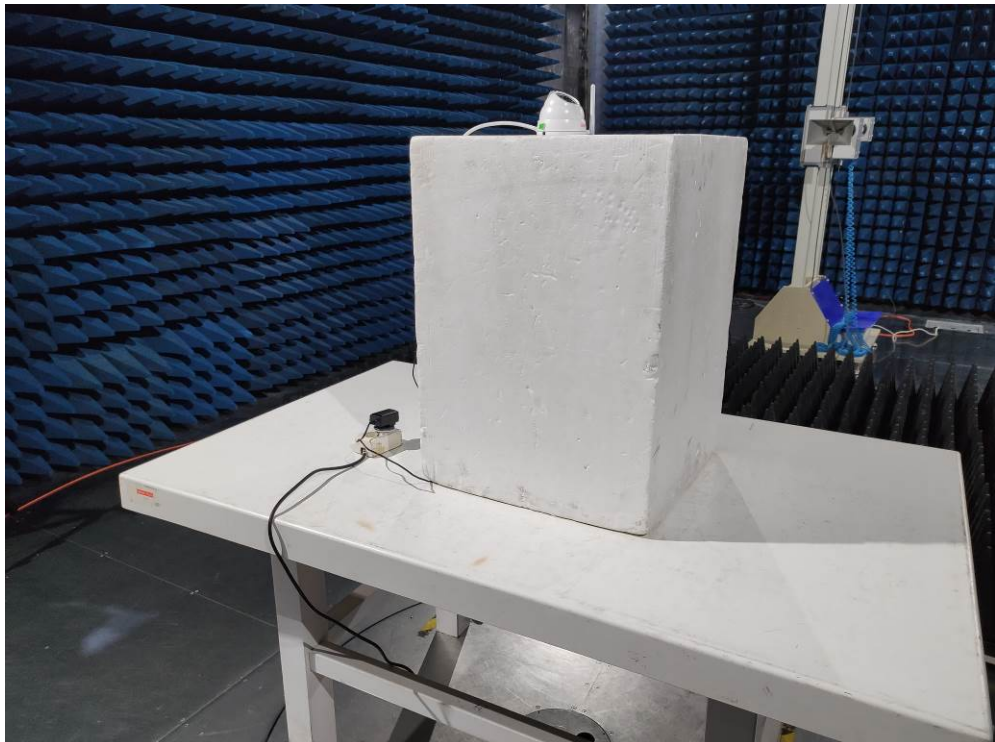
For Above 1GHz test site 1#
