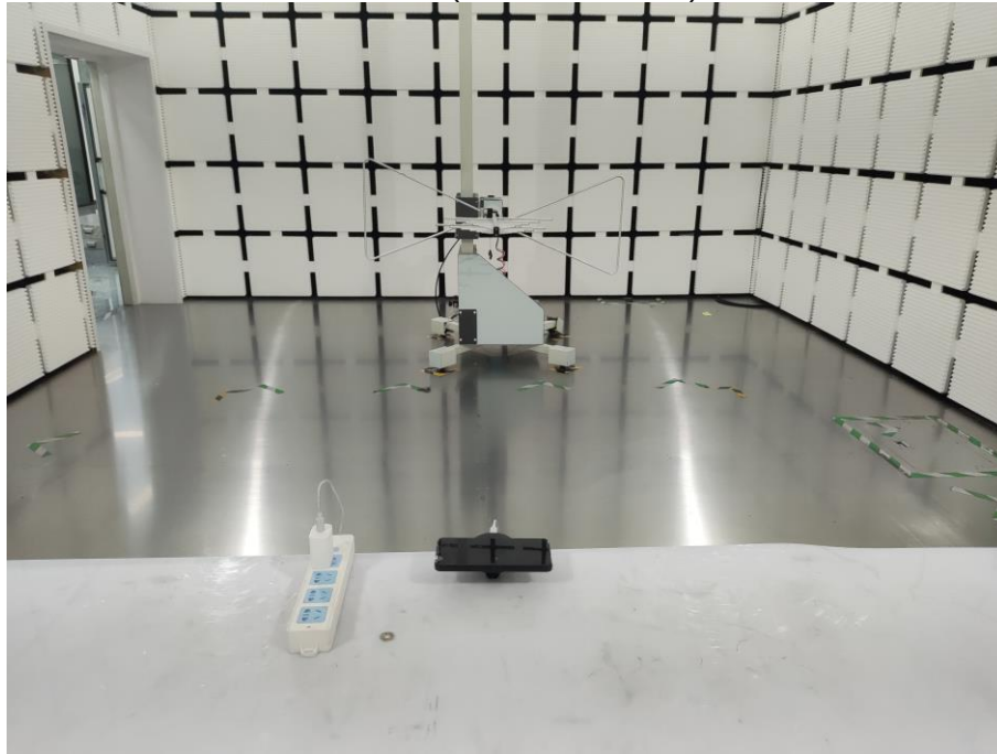
Radiation (30MHz-1000MHz)
