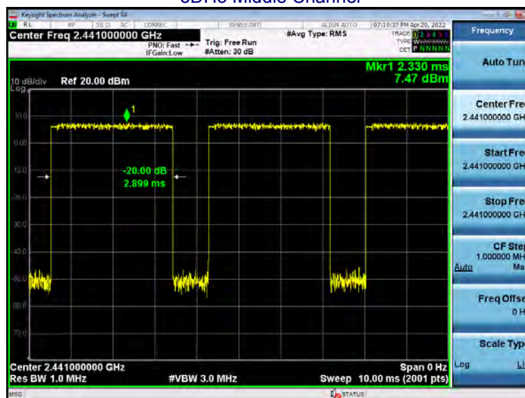
3DH5 Middle Channel
