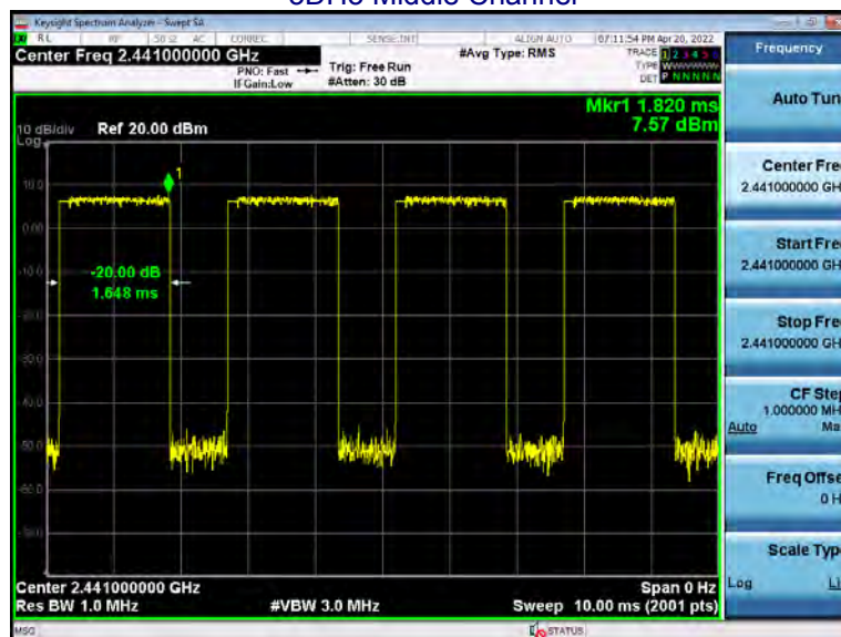
3DH3 Middle Channel
