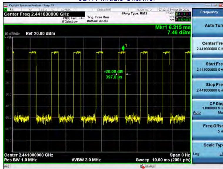
3DH1 Middle Channel
