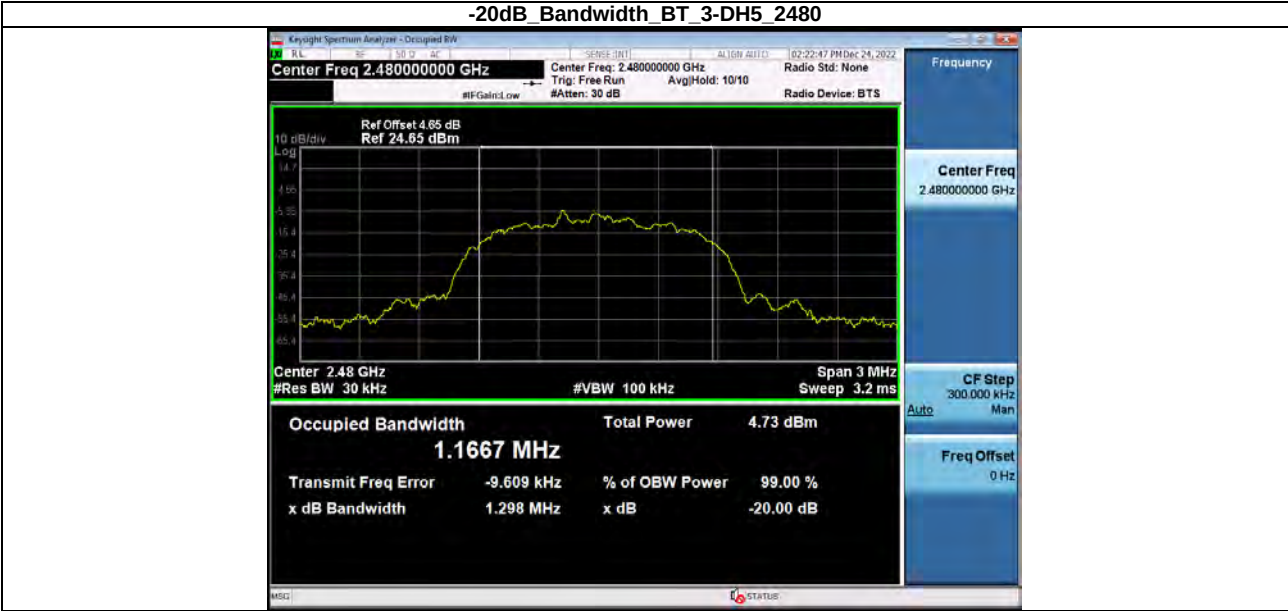
-20dB Bandwidth_BT_3-DH5_2480
