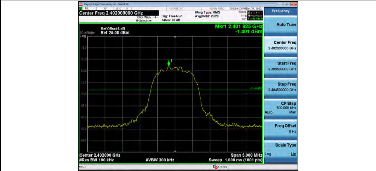
2_Bandedge_BT_3-DH5_2402
