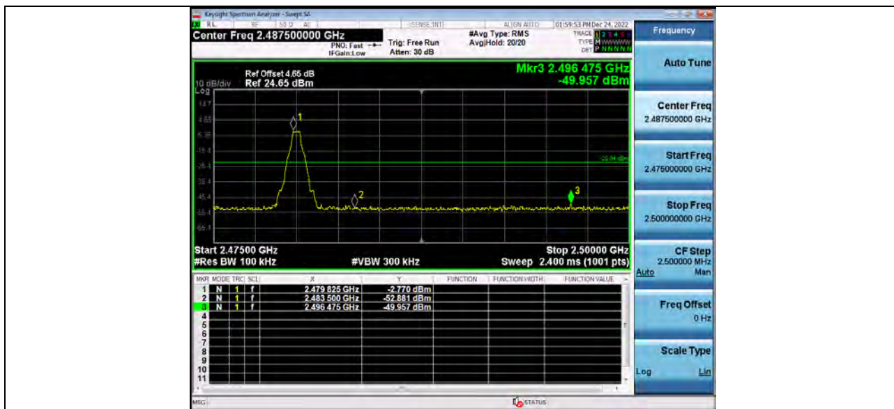
1 Reference Level BT 1-DH5 Hopping
