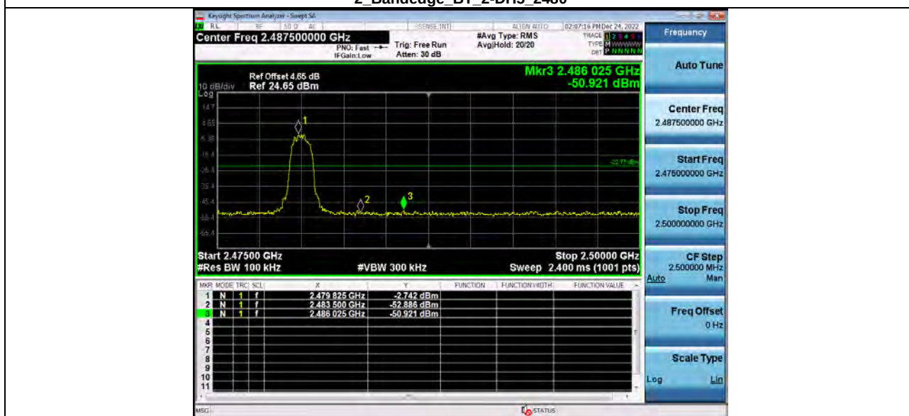
2. Bandedge BT 2-DH5 2480
