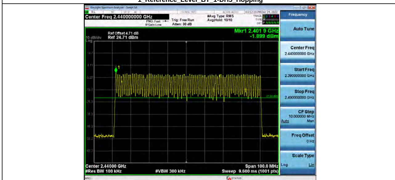
2 Band Edge (Hopping) BT 1-DH5 Hopping
