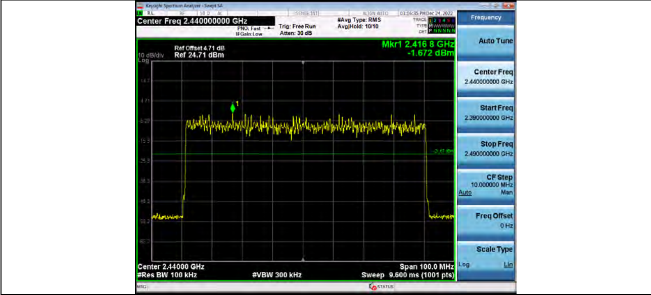
2_Band_Edge_(Hopping)_BT_2-DH5_Hopping
