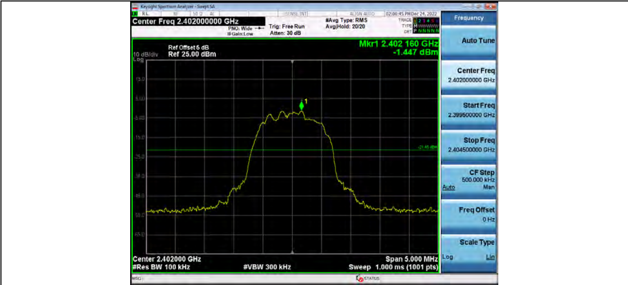
2_Bandedge_BT_2-DH5_2402
