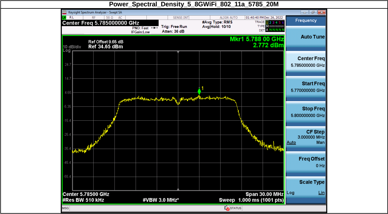
Power Spectral Density 5 8GWiFi 802 11a 5825 20M
