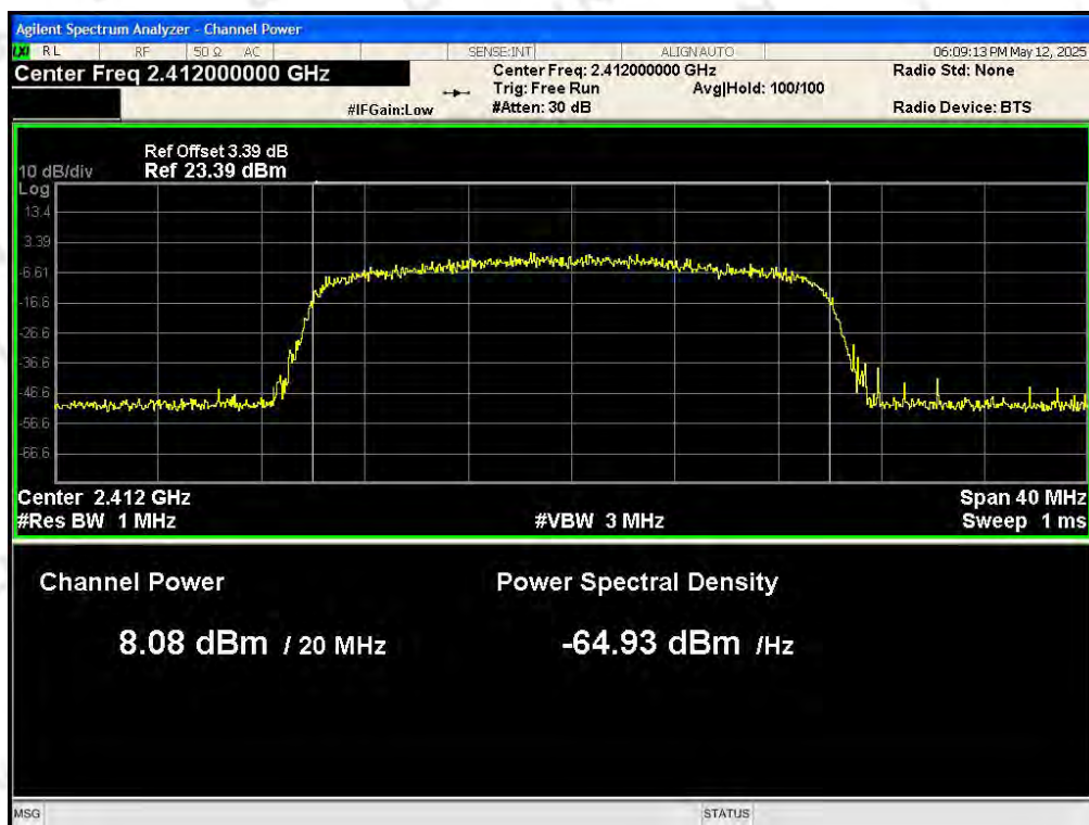
Power NVNT 802.11ax20 2412MHz Ant0
