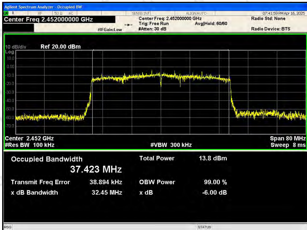
OBW NVNT 802.11ax40 2452MHz Ant1
