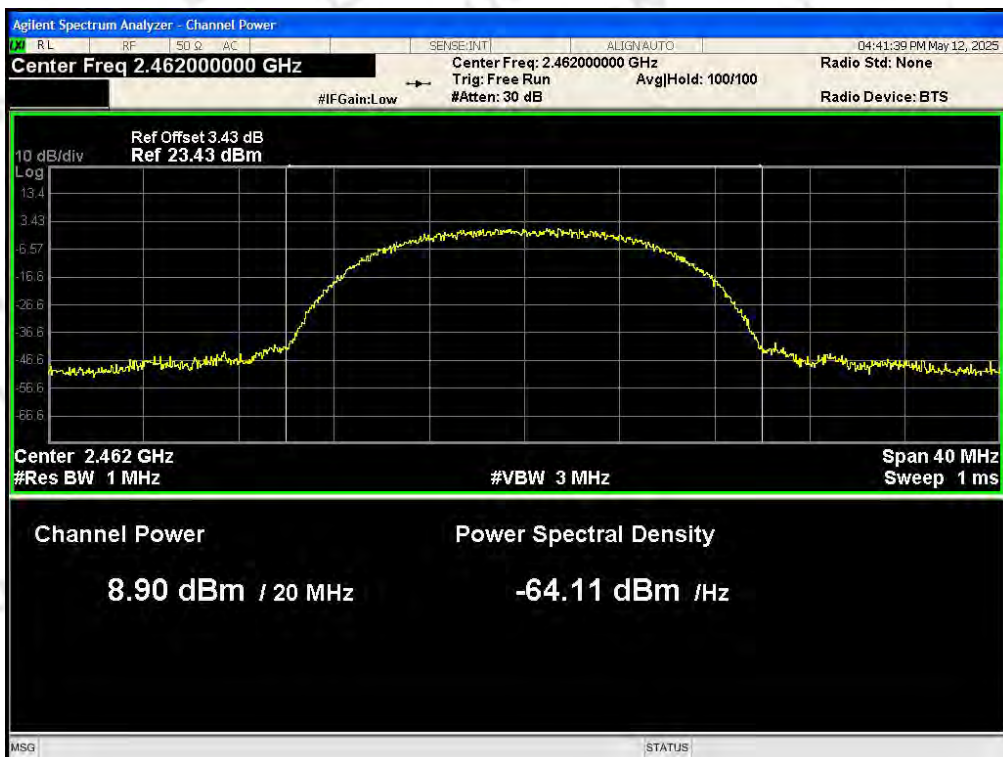
Power NVNT 802.11b 2462MHz Ant0
