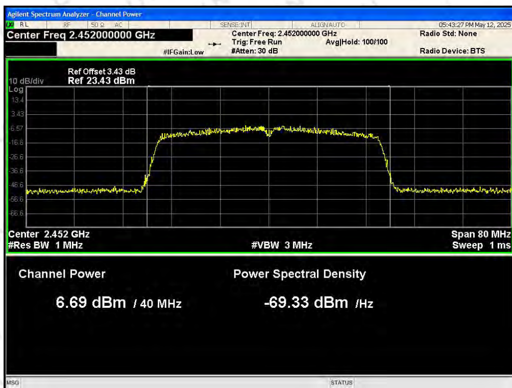
Power NVNT 802.11n(HT40) 2452MHz Ant1
