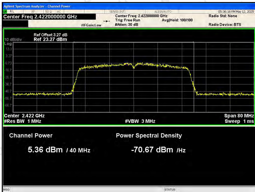
Power NVNT 802.11n(HT40) 2422MHz Ant1
