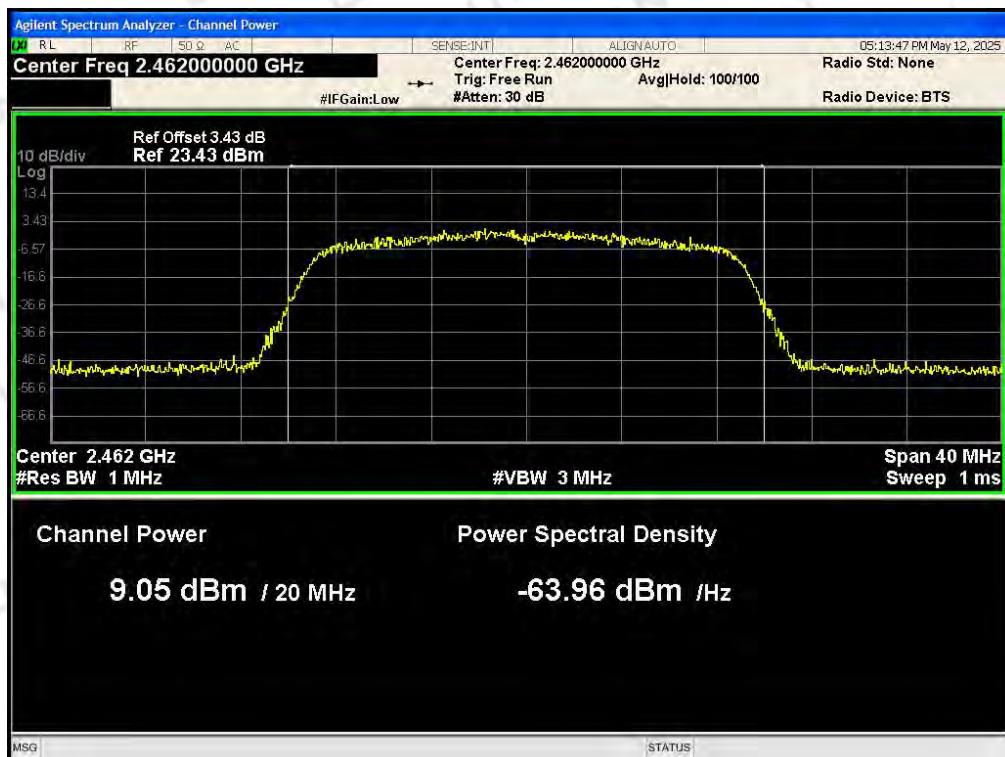
Power NVNT 802.11n(HT20) 2462MHz Ant0
