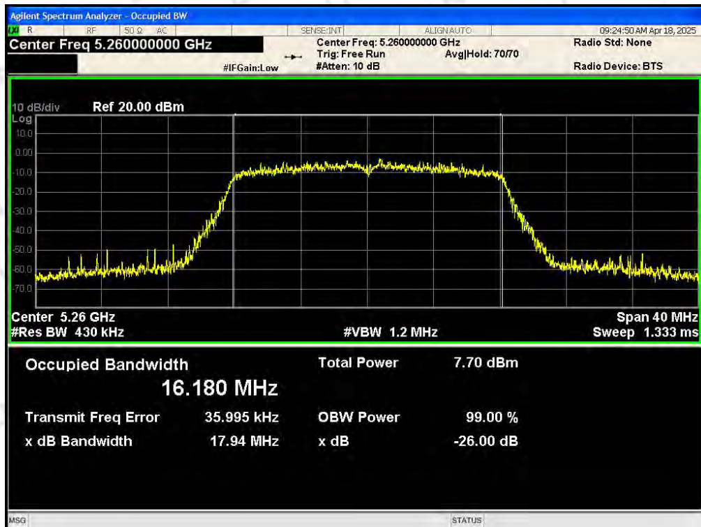
-26 dB Bandwidth NVNT 802.11a 5260MHz Ant1
