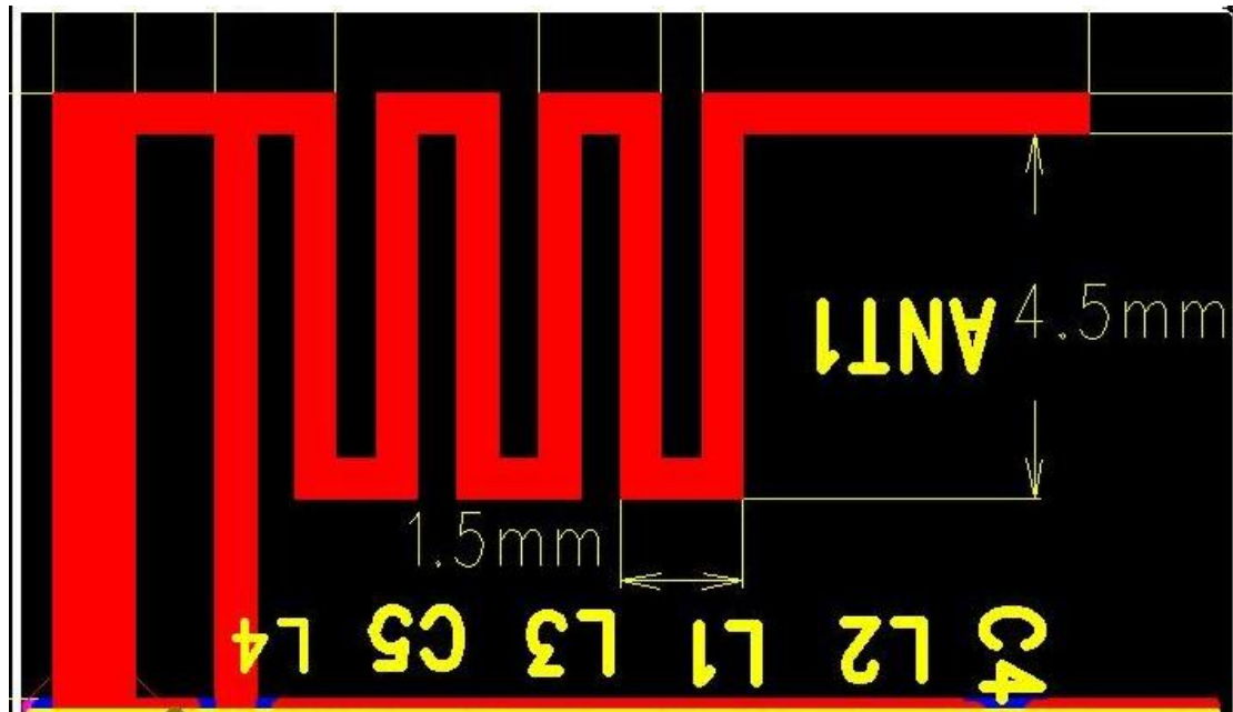
2-1 Normal Dongle PIFA Antenna
