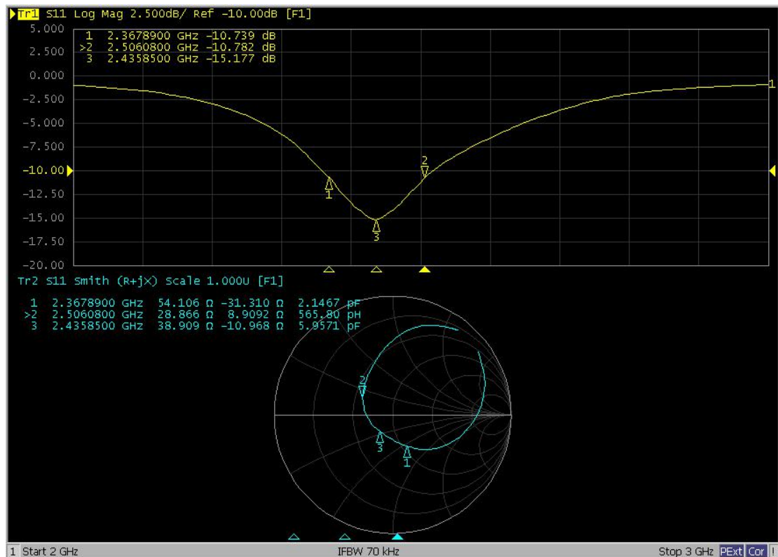
2-2 Normal Dongle PIFA S11 performance
