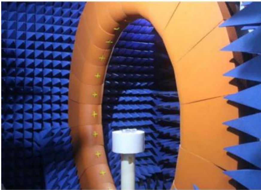
Anechoic chamber
