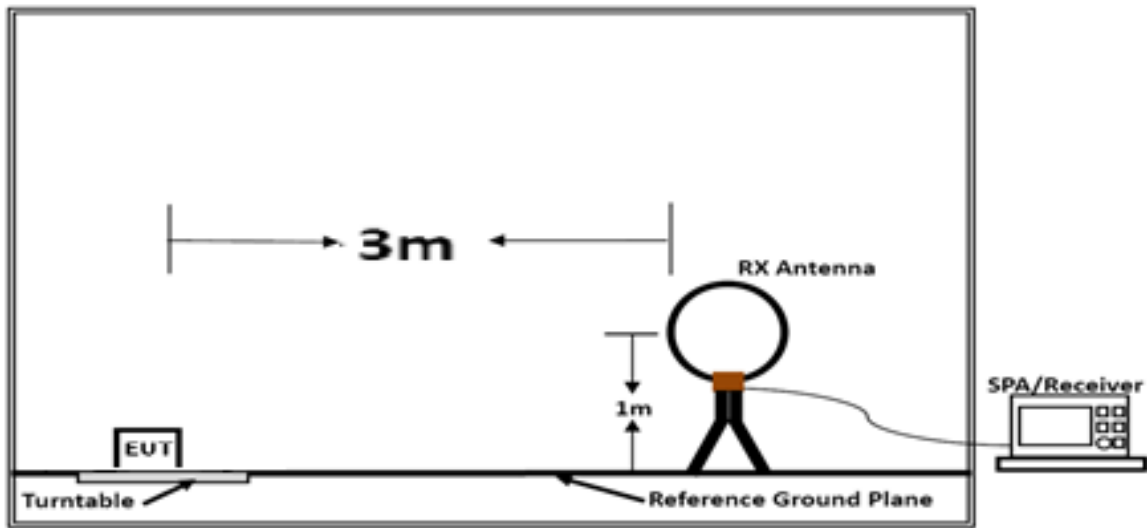
Below 30MHz
