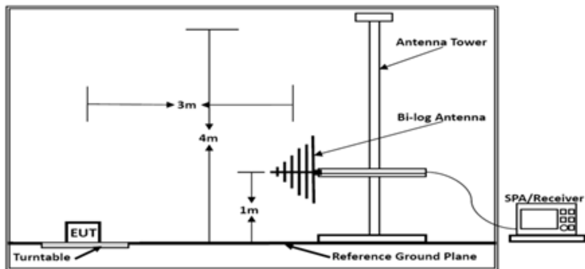
Below 1GHz
