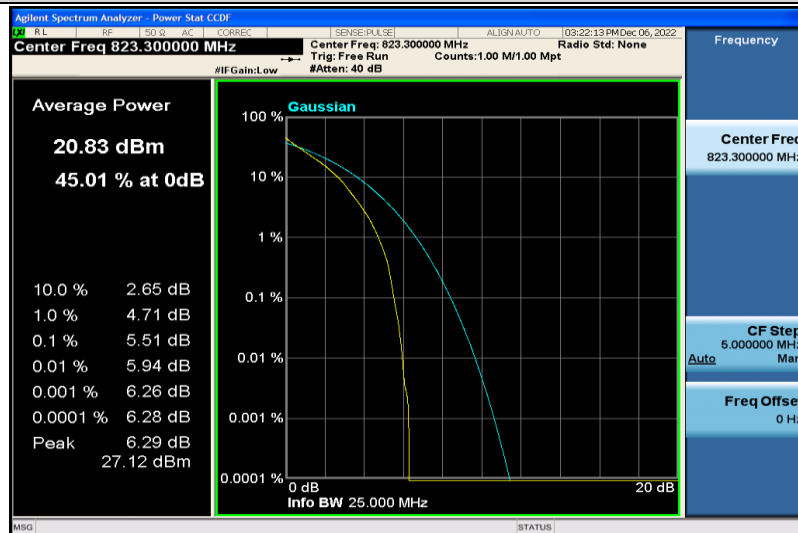
Band26-1.4MHz-QPSK-26783-6RB#0
