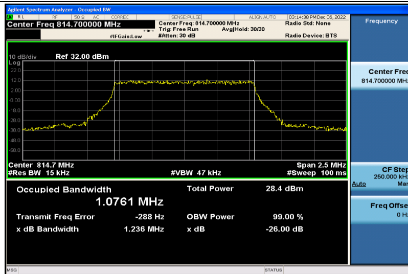
Band26-1.4MHz-QPSK-26697-6RB#0-1.0761
