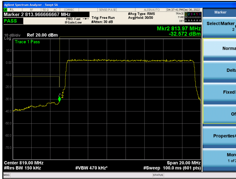
Band26-15MHz-QPSK-26765-75RB#0
