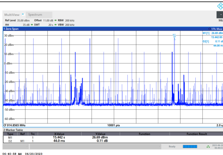
2GFSK-150 kbps _Ant1_Hop- The number of hop channel appear
