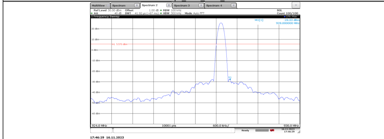
2GFSK-25 kbps_Ant1_HCH_Bandedge
