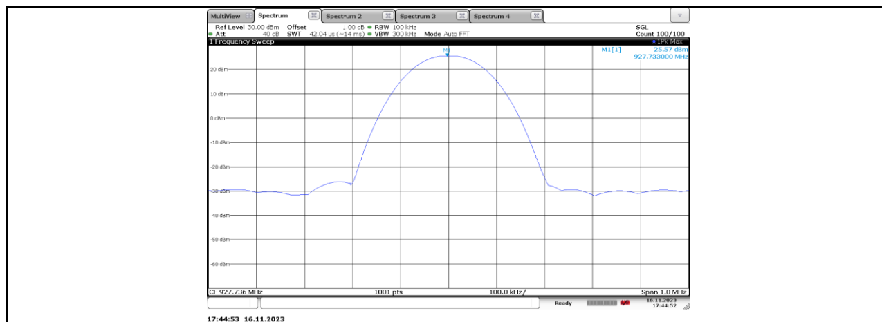
2GFSK-25 kbps_Ant1_HCH_Reference
