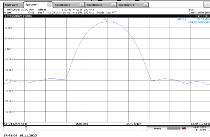
2GFSK-25 kbps Ant1 MCH_Reference
