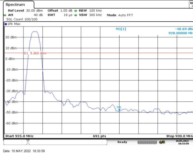
2GFSK-75 kbps_Ant1_HCH_Bandedge
