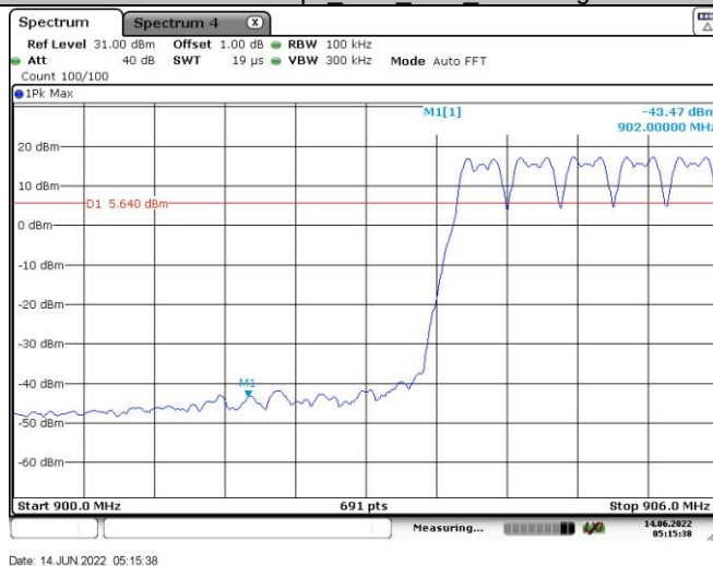
2GFSK-250 kbps_Ant1_LCH_Bandedge Hopping on
