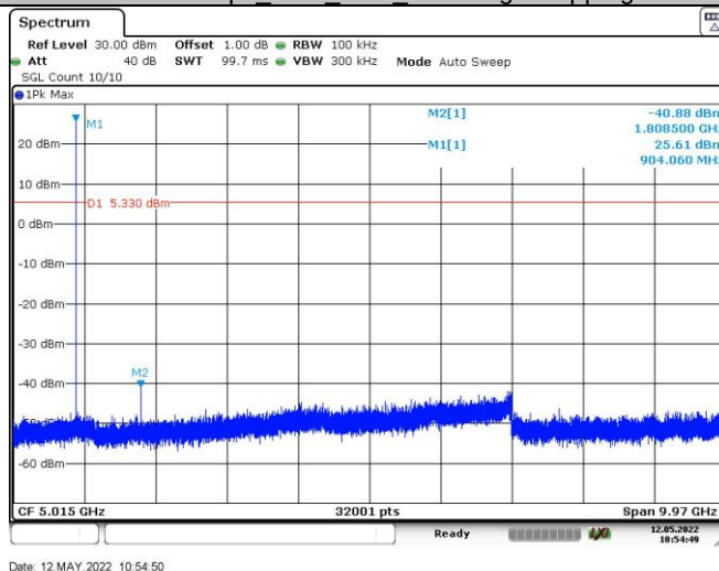
2GFSK-75 kbps_Ant1_LCH_Spurious
