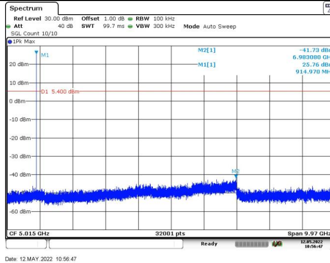
2GFSK-75 kbps_Ant1_MCH_Spurious
