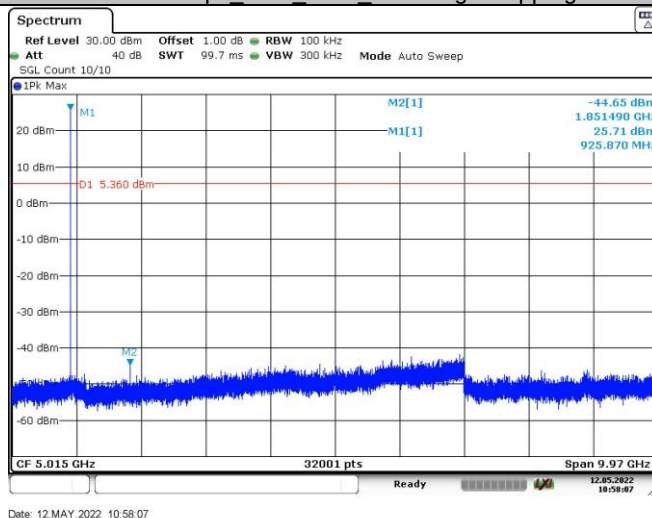
2GFSK-75 kbps_Ant1_HCH_Spurious
