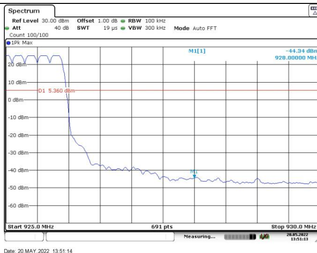
2GFSK-75 kbps_Ant1_HCH_Bandedge Hopping on
