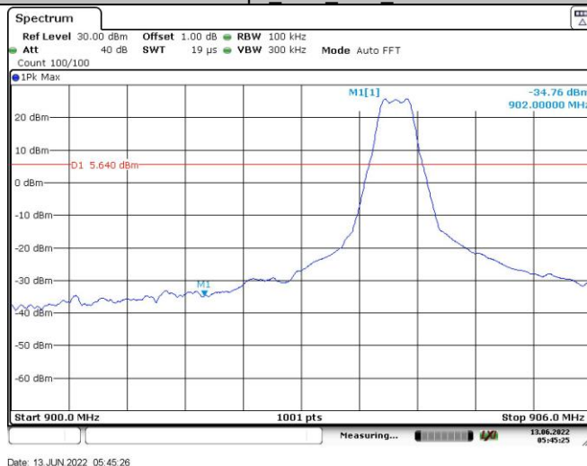
2GFSK-250 kbps_Ant1_LCH_Bandedge
