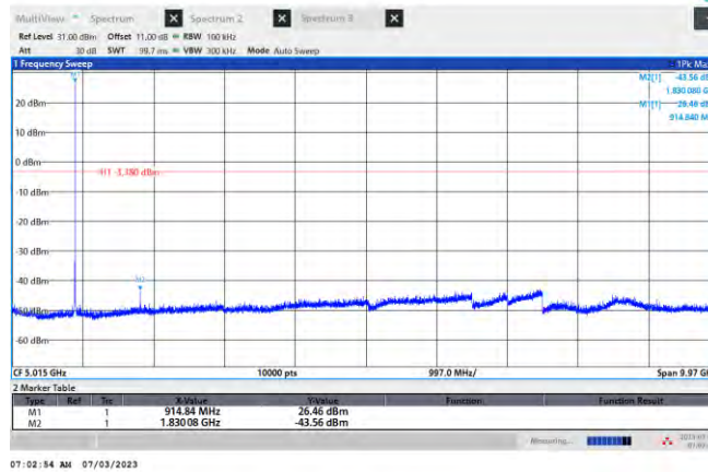
2GFSK.640kbps_Ant1_MCH
