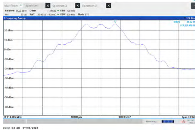
2GFSK.640kbps_Ant1_MCH
