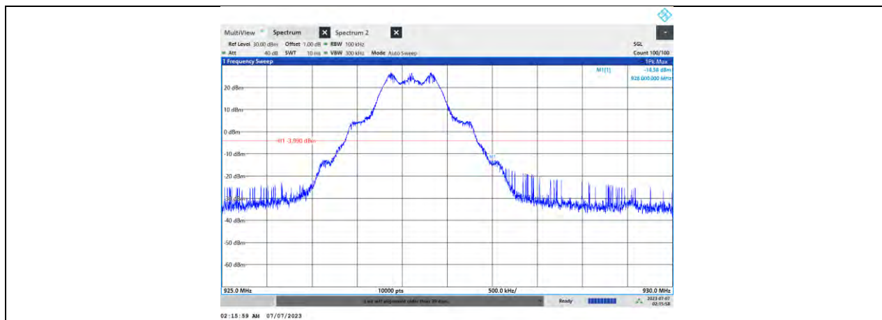
2GFSK.640kbps_Ant1_HCH
