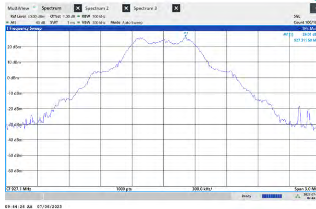
2GFSK.640kbps_Ant1_HCH
