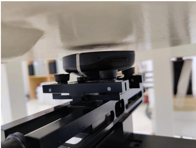
Left Side (5mm)-WiFi/BT Ant
