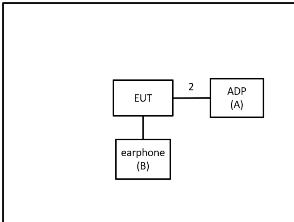
Radiated Emissions
