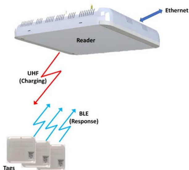
Figure 2 - Reader's functionality
