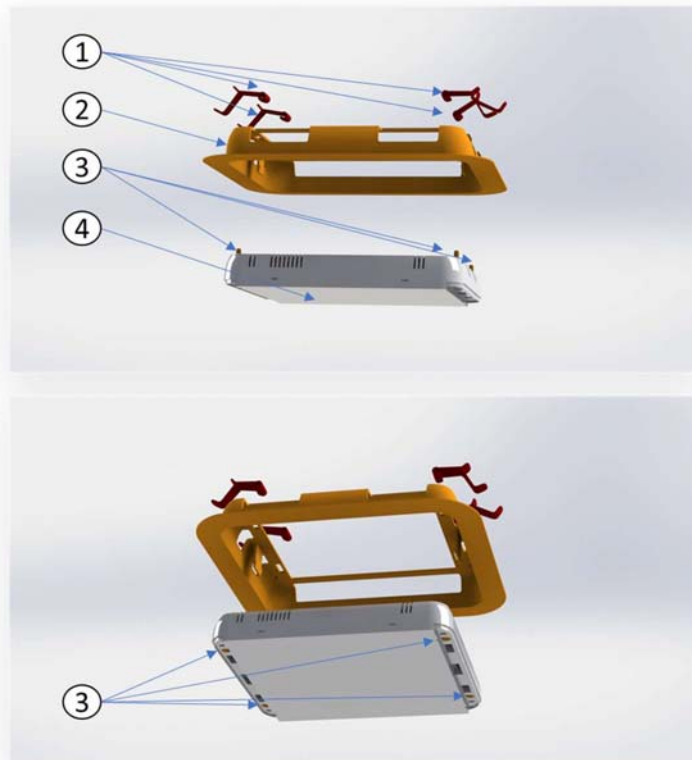
Figure 9 - Flush mounting kit – Installation illustration
