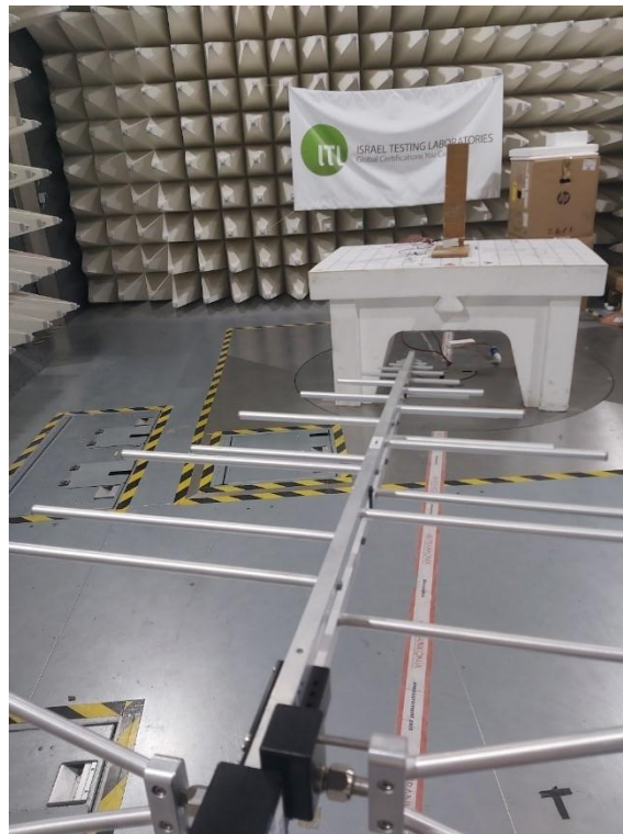
Figure 1 30MHz-1GHz
