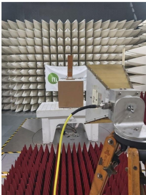
Figure 4 1GHz-8GHz
