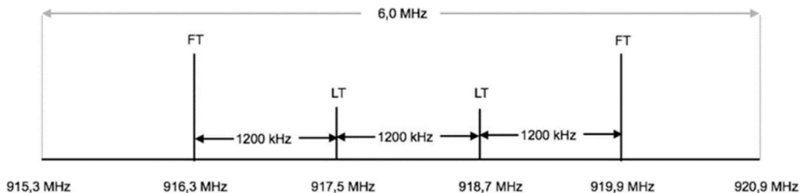
Figure 6 – EN 302 308 Upper band designated frequencies
