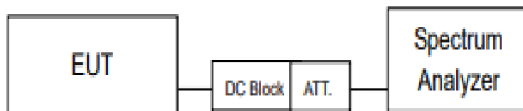
Figure 23: Typical test setup for Power Spectral Density
