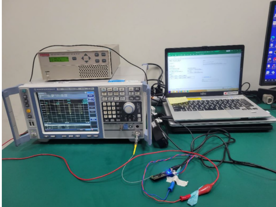
Photograph 9: Test Setup for Conducted
