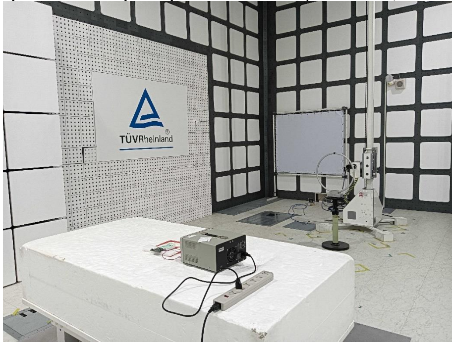
Photograph 12: Test Setup for Spurious Emissions (Back View 2, Ant No.: 2 & 3)
