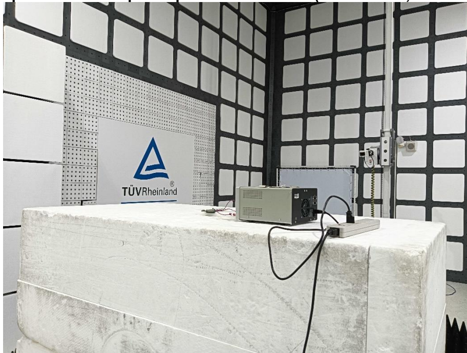
Photograph 14: Test Setup for Spurious Emissions (Back View 4, Ant No.: 2 & 3)
