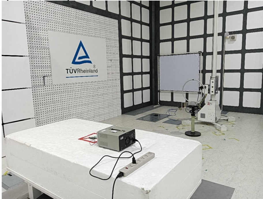
Photograph 4: Test Setup for Spurious Emissions (Back View 2, Ant No.: 1)
