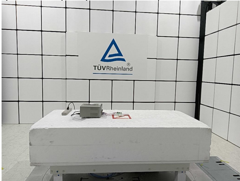
Photograph 10: Test Setup for Spurious Emissions (Front View 2, Ant No.: 2 & 3)
