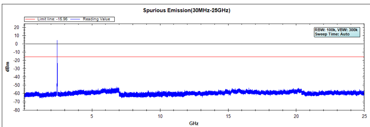
Channel 11 (2462MHz)
