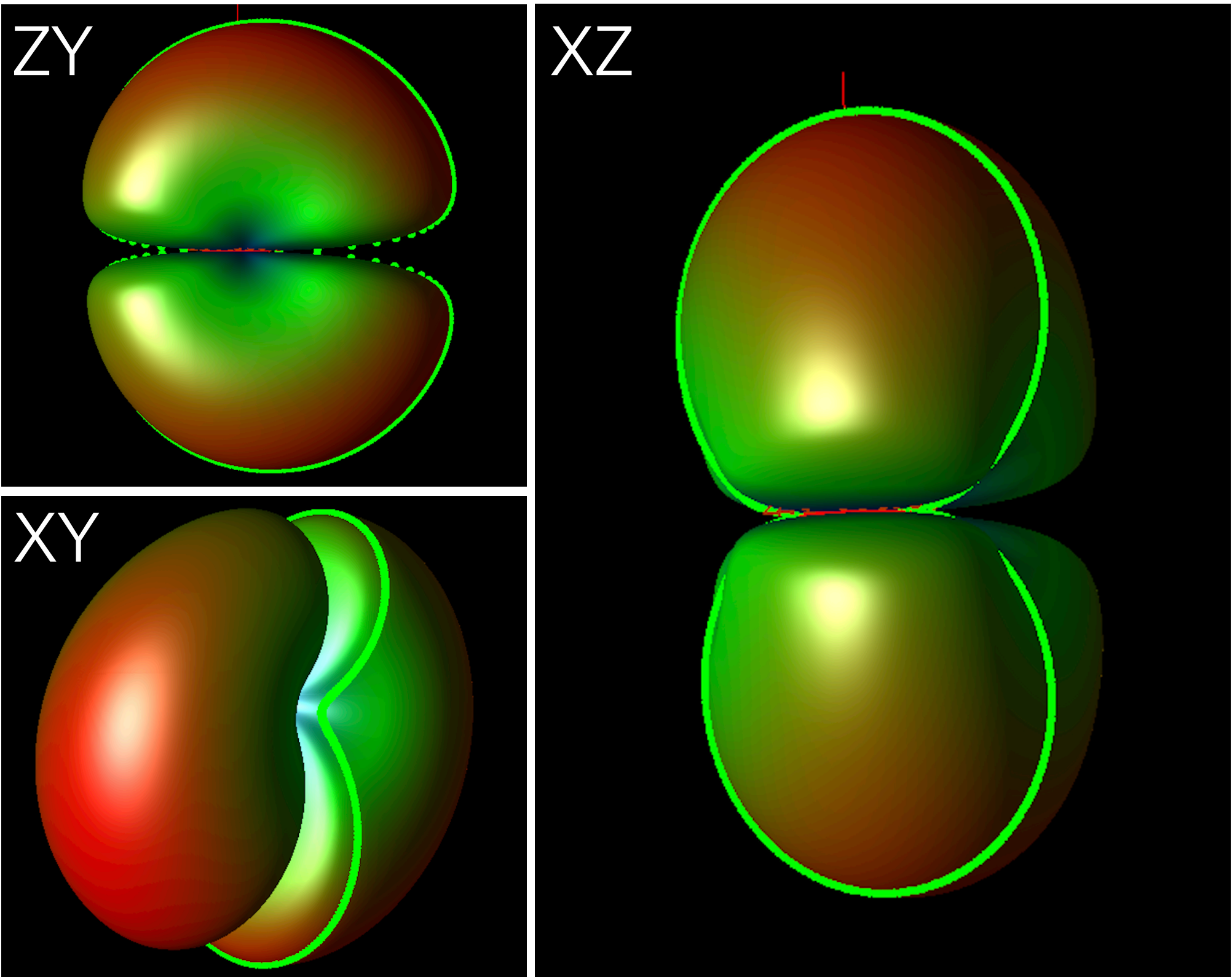
Gain Pattern
