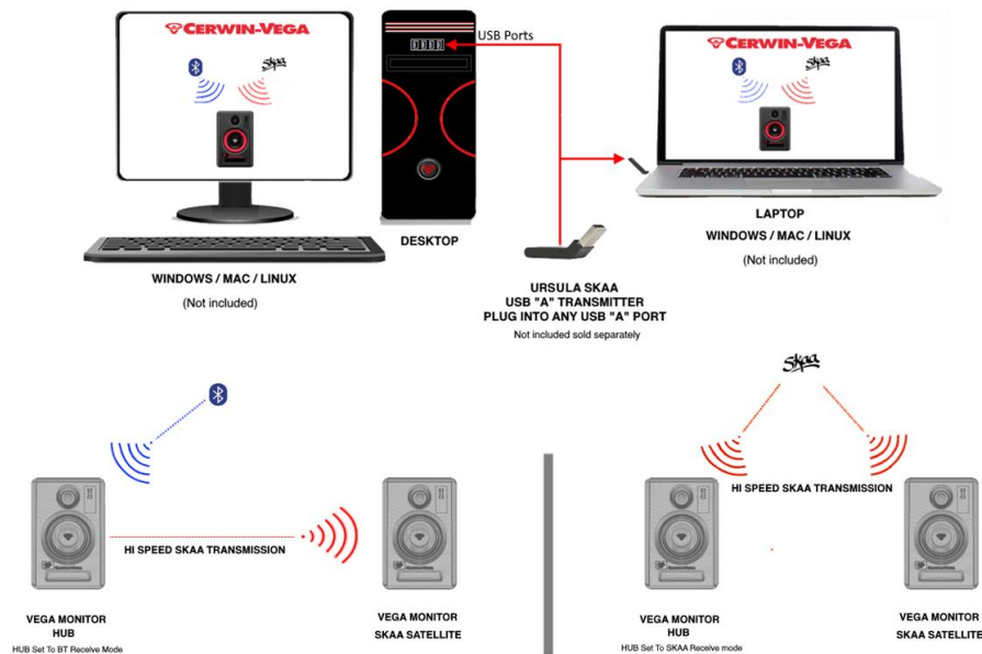
Figure 3: Computer or BT source or SKAA Connections to Monitor
