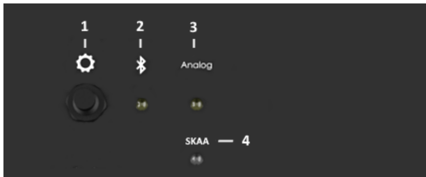
Figure 1: HUB Input Audio Connection Controls
