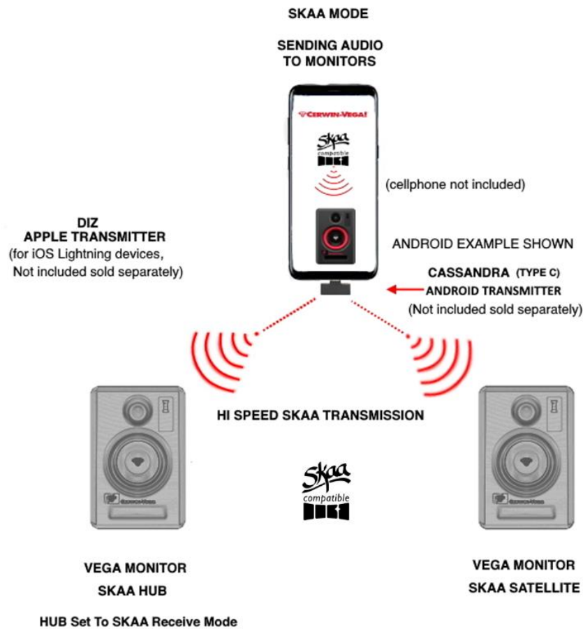
Figure 5: Cellphone connection to Monitor using SKAA mode.
