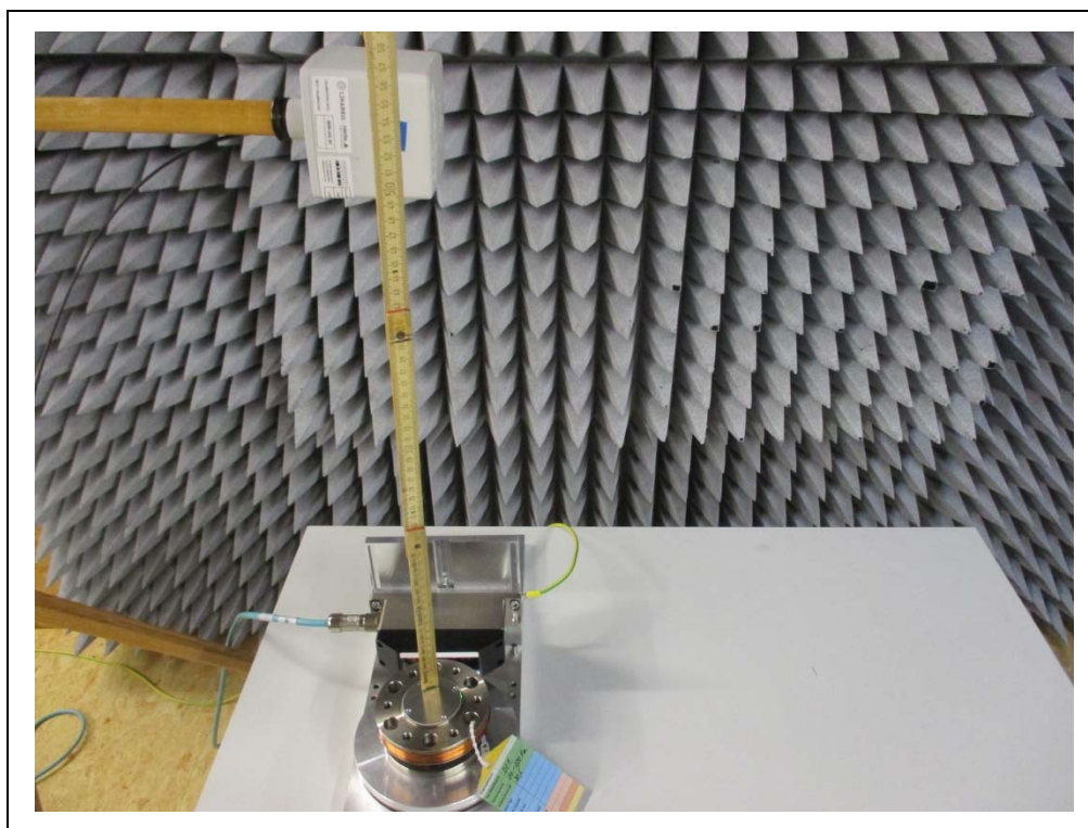
Photograph A1-2: SETUP B (distance from surface of EUT to surface of probe)
