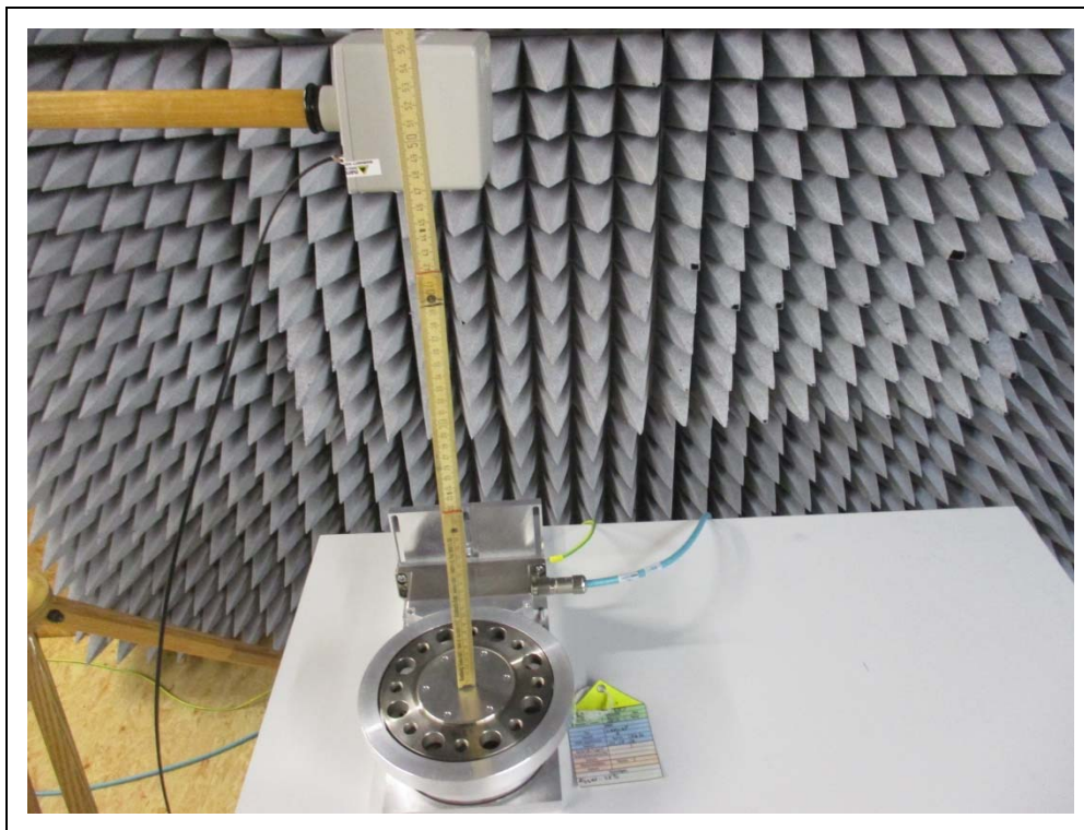
Photograph A1-1: SETUP A (distance from surface of EUT to center of probe)
