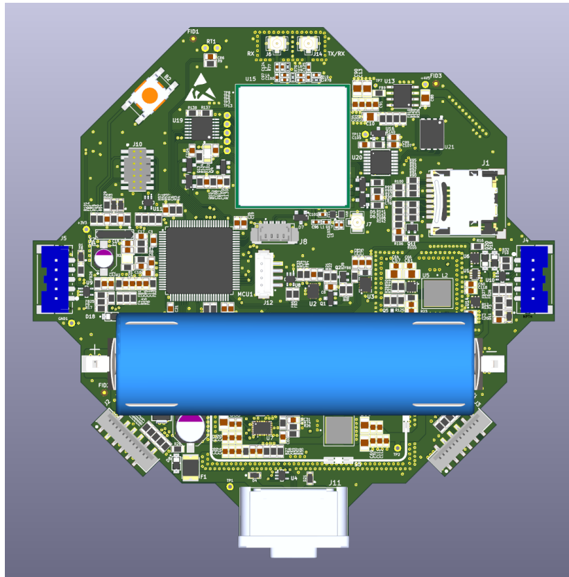
MAIN PCB- FRONT VIEW
