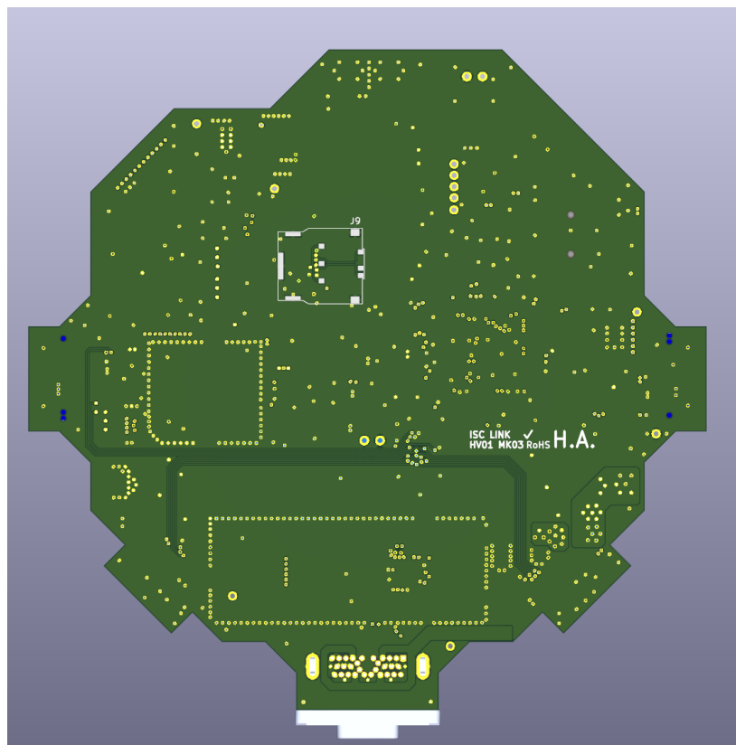
MAIN PCB- BACK VIEW
